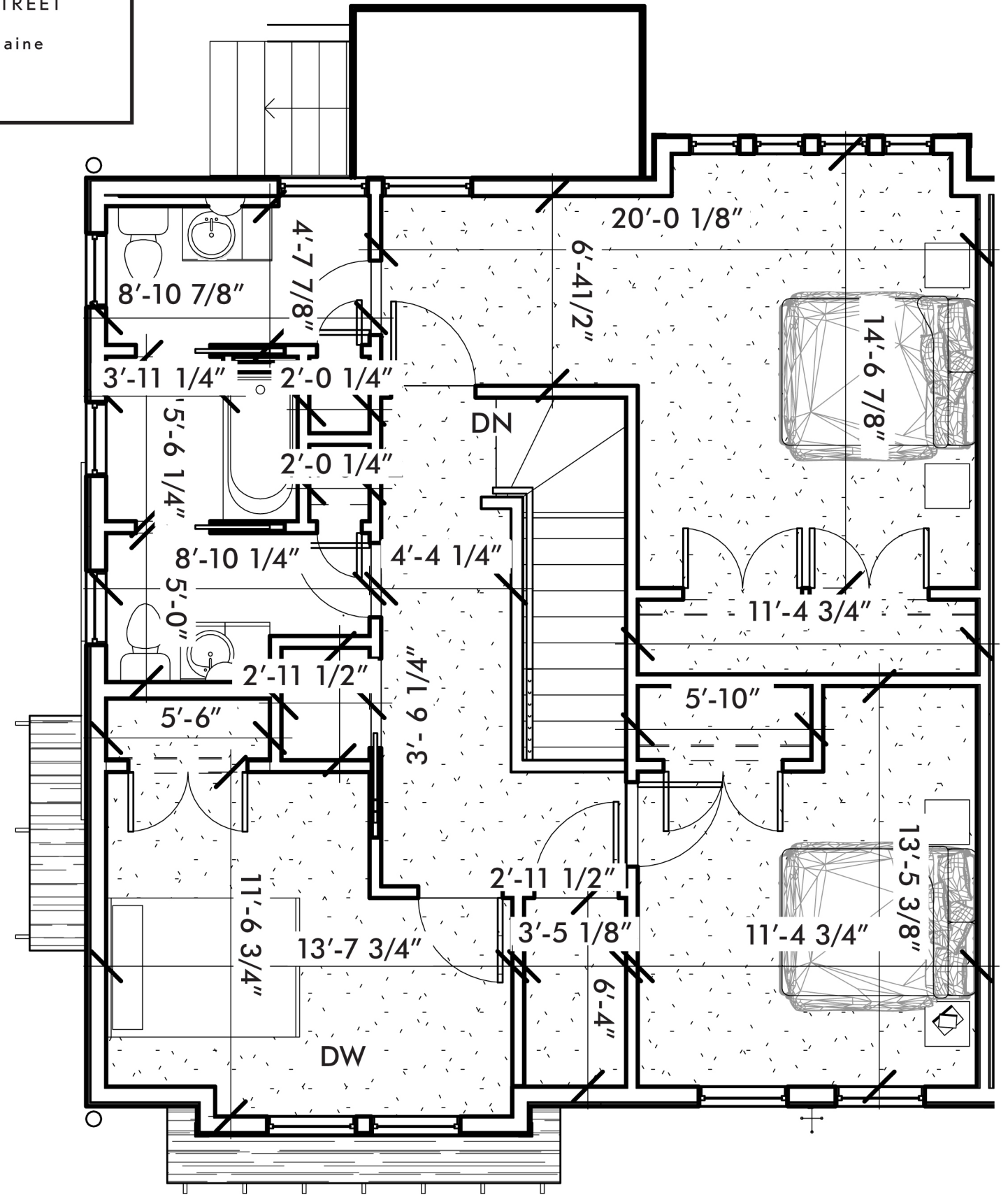
2 ADAMS SCHOOL CONDOMINIUMS - UNIT PLAN E - 2nd Floor
