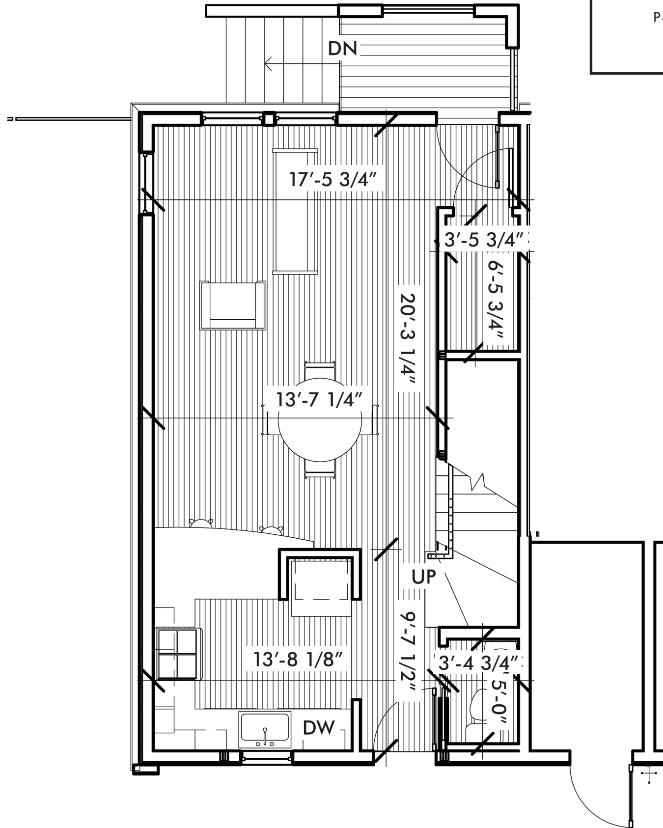
1 ADAMS SCHOOL CONDOMINIUMS - UNIT PLAN E - 1st Floor
