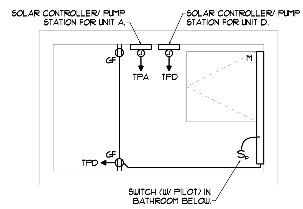
ALTERNATE #4 - ATTIC MECHANICAL ROOM SCALE: 1/2" = 1'-0"
