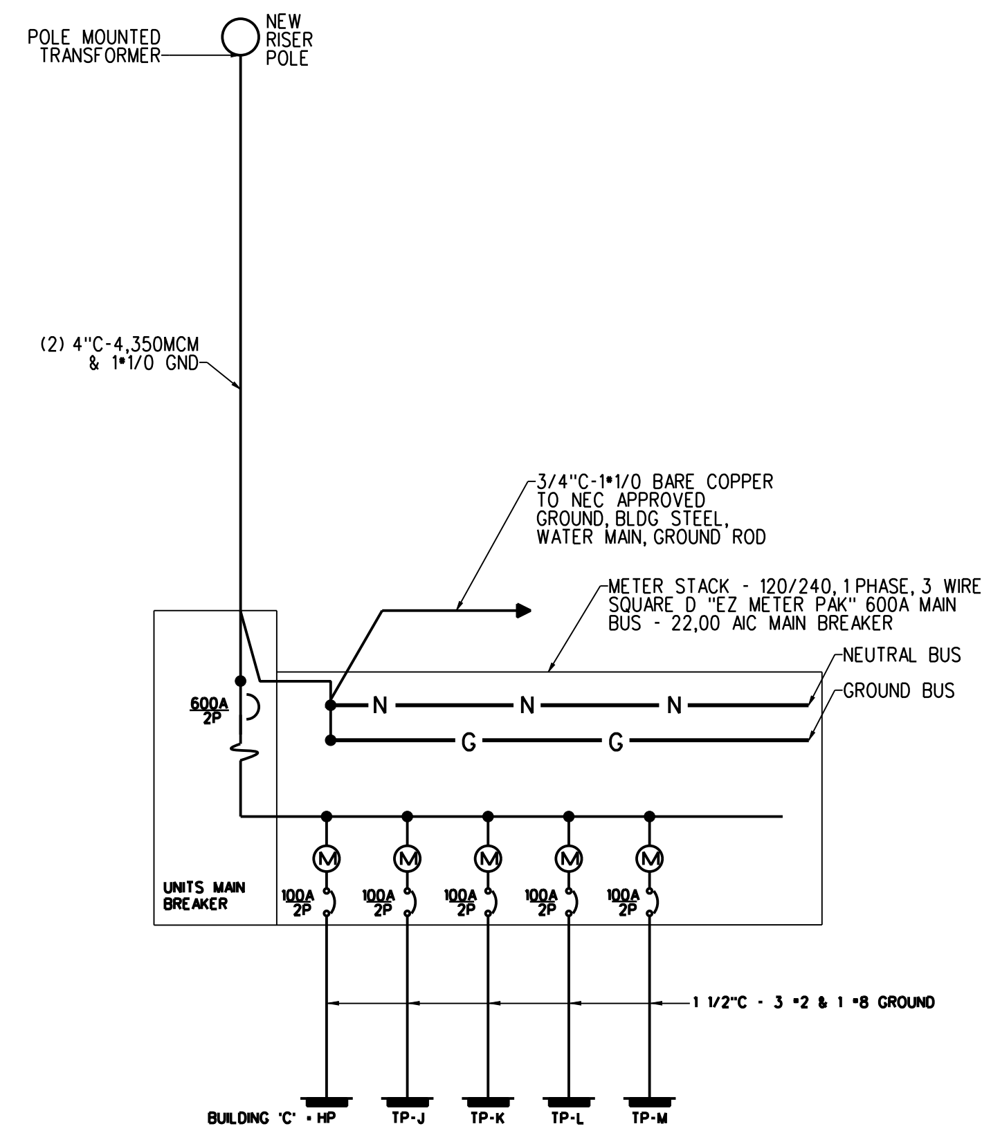
BUILDING 'C' ONE LINE DIAGRAM SCALE: NONE
