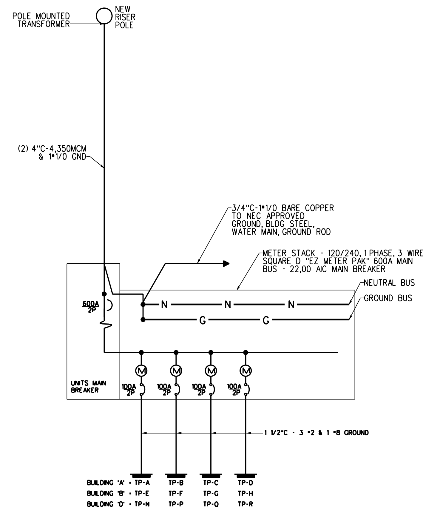
BUILDINGS 'A', 'B' & 'D' ONE LINE DIAGRAM SCALE: NONE
