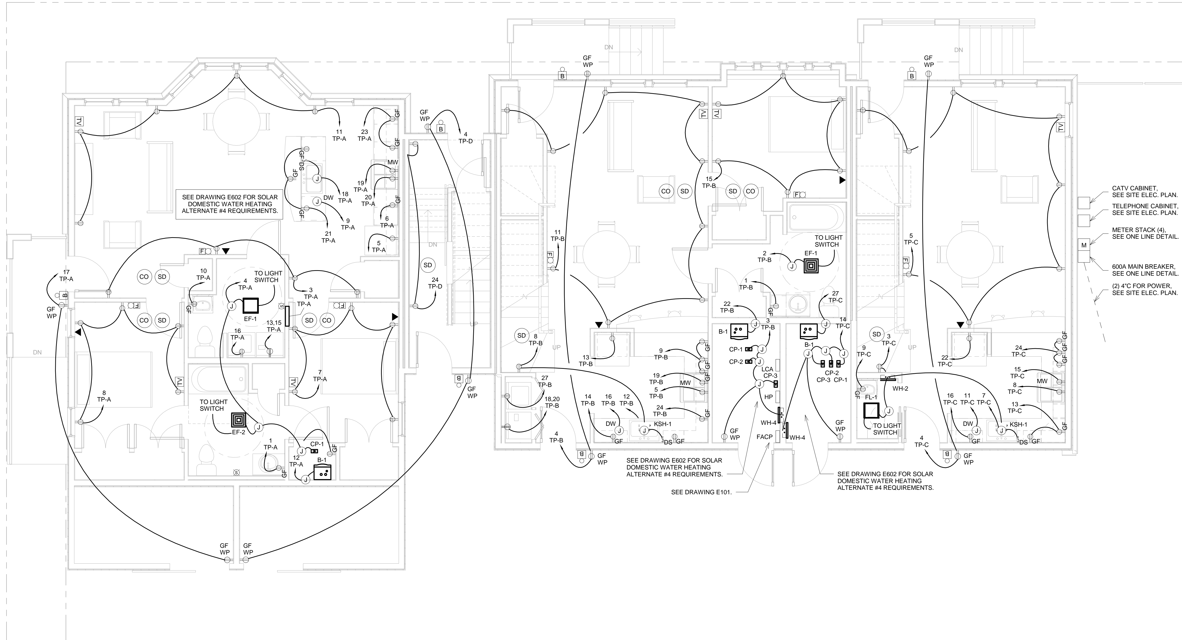
1 Bldg A 1st Flr Power Plan 1/4" = 1'-0"
