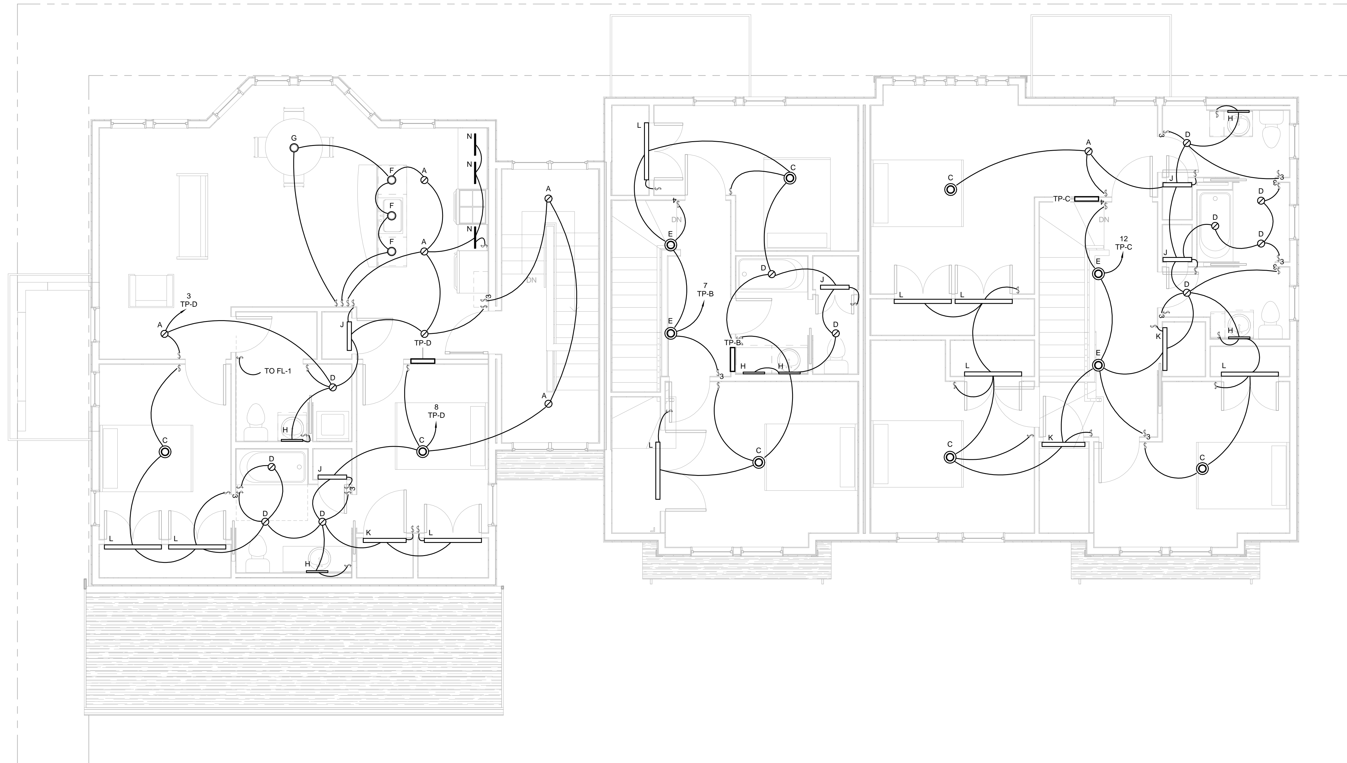
1 Bldg A 2nd Flr Lighting Plan 1/4" = 1'-0"
