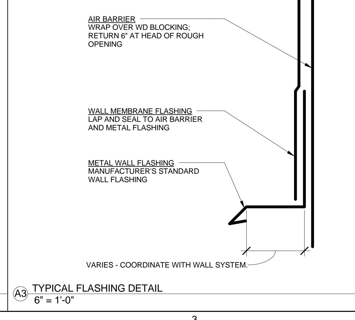
A3 TYPICAL FLASHING DETAIL 6" = 1'-0"
