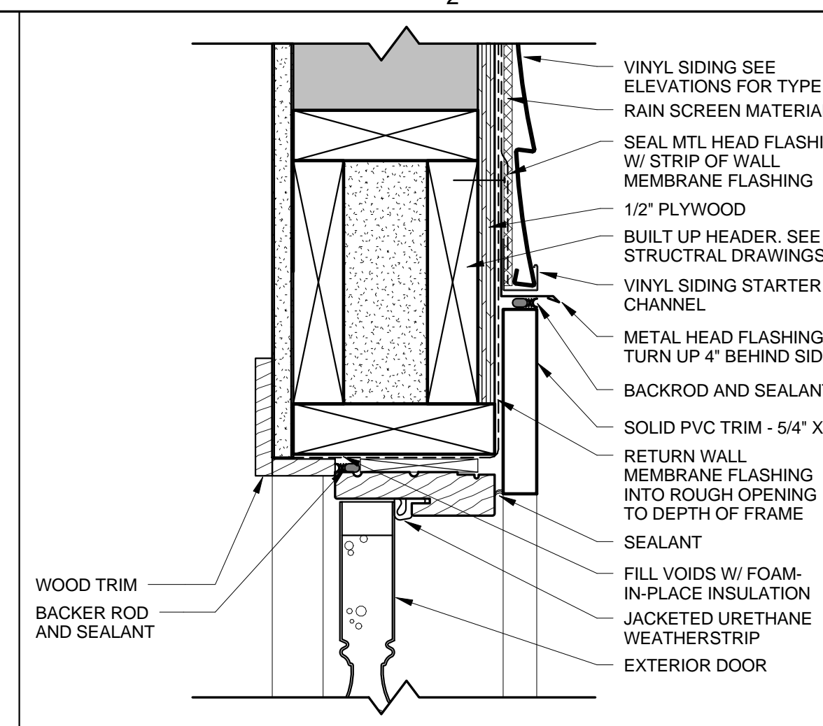
D2 EXTERIOR DOOR HEAD DETAIL 3" = 1'-0"
