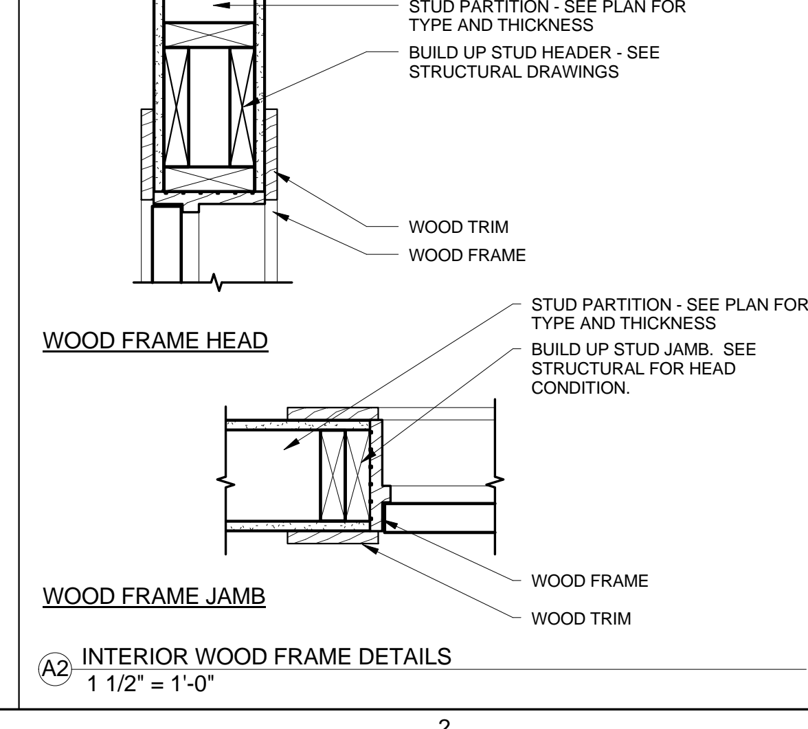
A2 INTERIOR WOOD FRAME DETAILS 1 1/2" = 1'-0"
