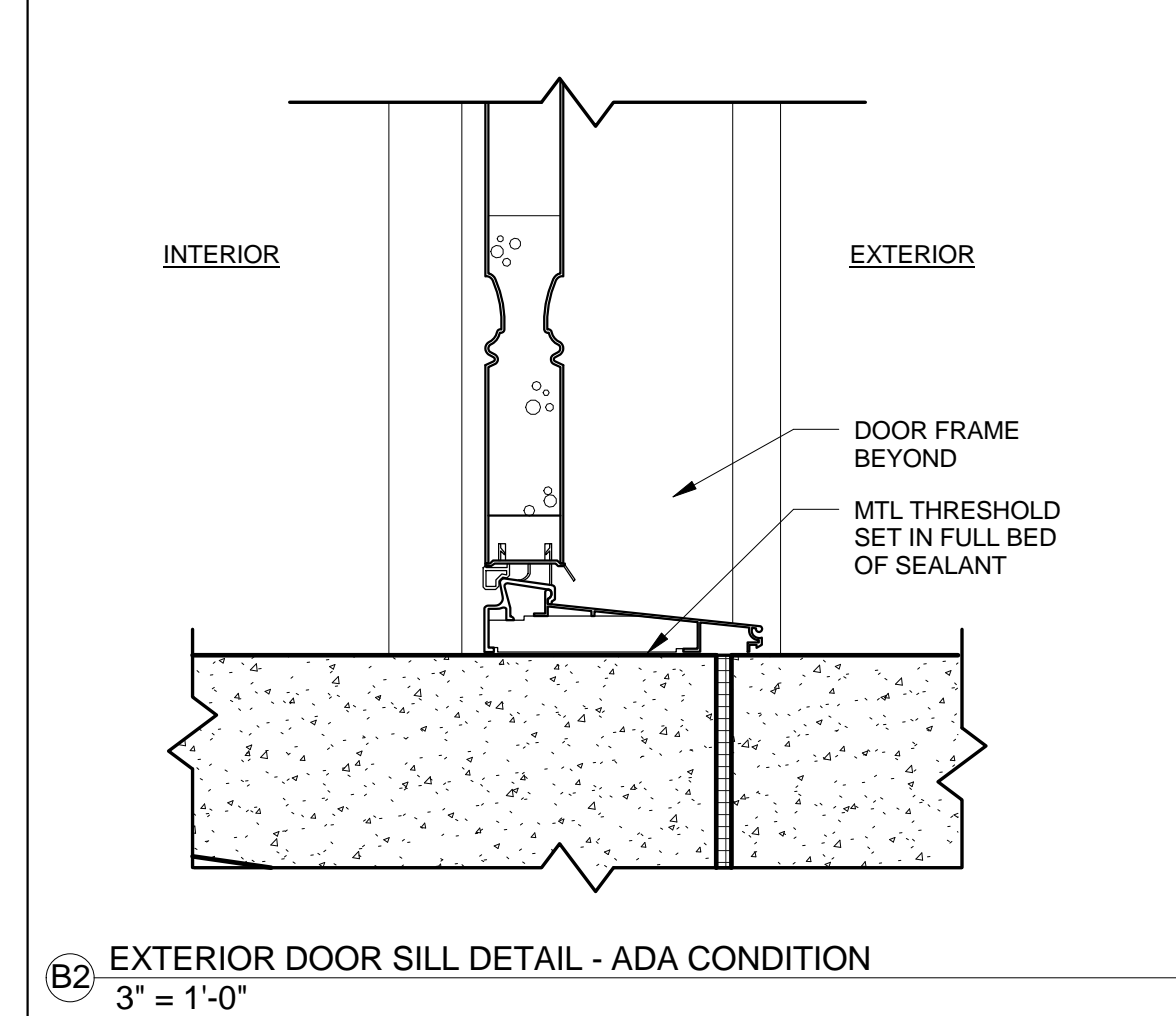
B2 EXTERIOR DOOR SILL DETAIL - ADA CONDITION 3" = 1'-0"
