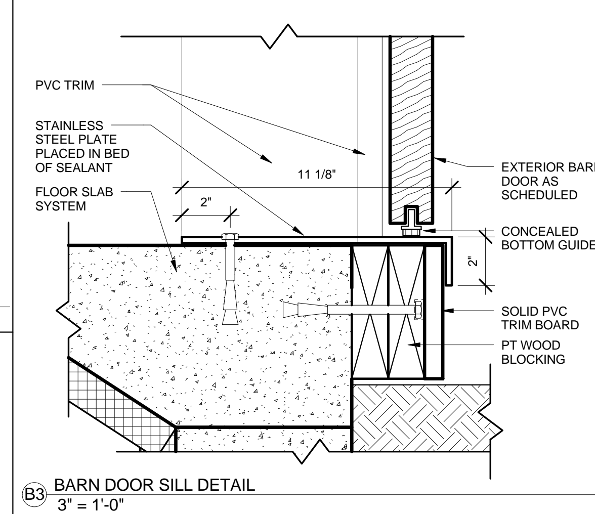
B3 BARN DOOR SILL DETAIL 3" = 1'-0"
