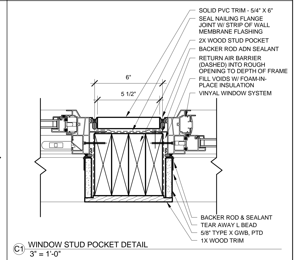
C1 WINDOW STUD POCKET DETAIL 3" = 1'-0"
