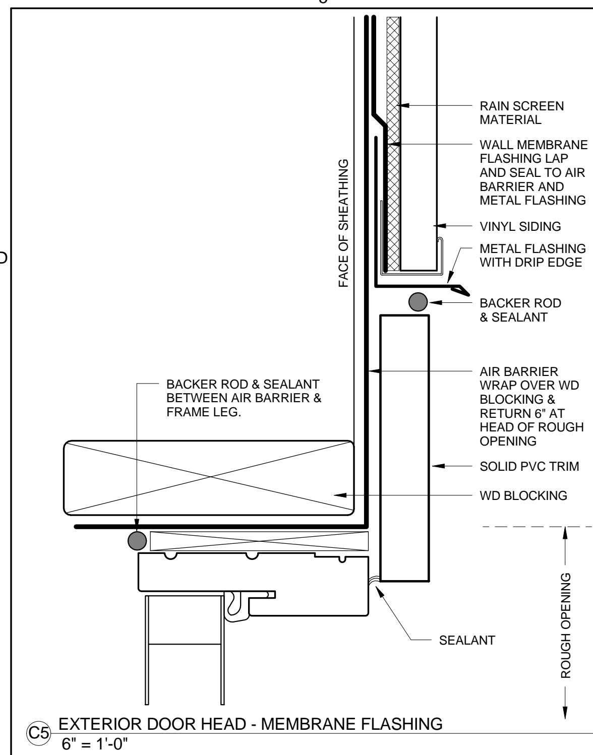
C5 EXTERIOR DOOR HEAD - MEMBRANE FLASHING 6" = 1'-0"
