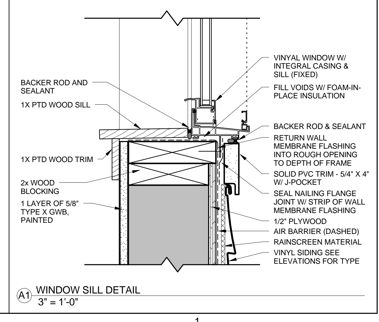
A1 WINDOW SILL DETAIL 3" = 1'-0"
