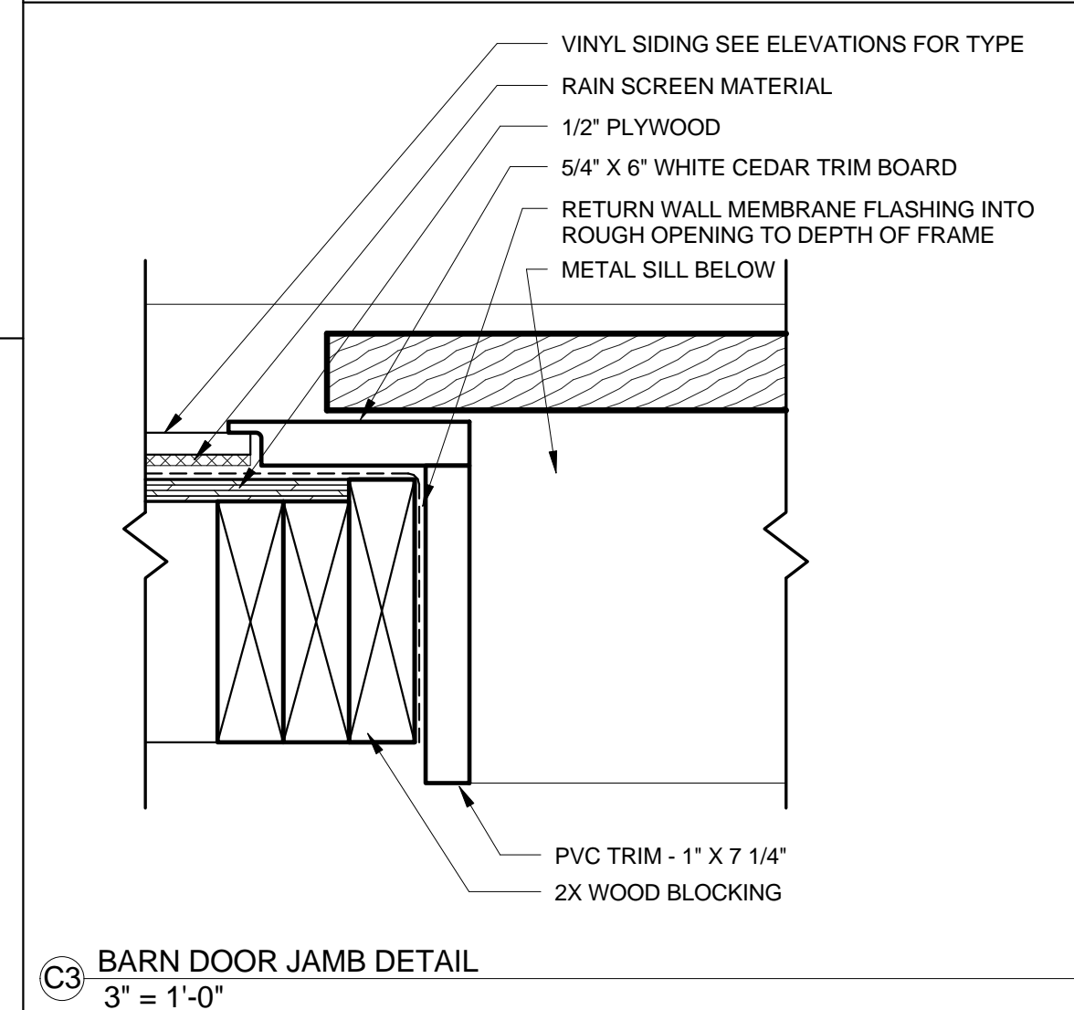
C3 BARN DOOR JAMB DETAIL 3" = 1'-0"
