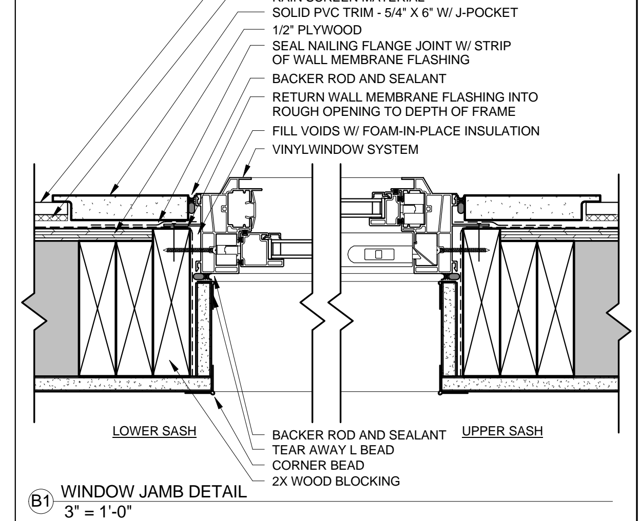
B1 WINDOW JAMB DETAIL 3" = 1'-0"
