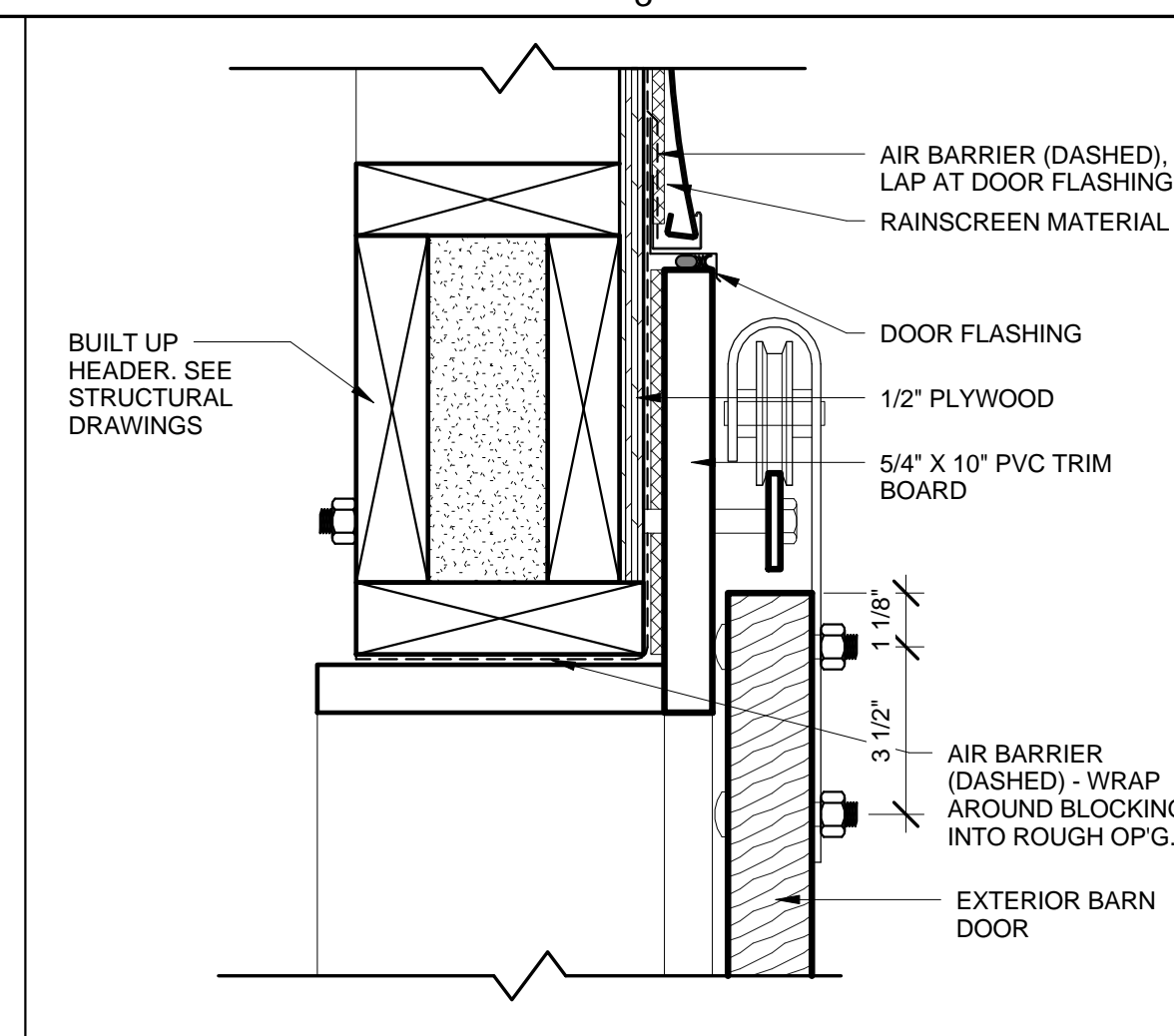
D3 BARN DOOR HEAD DETAIL 3" = 1'-0"
