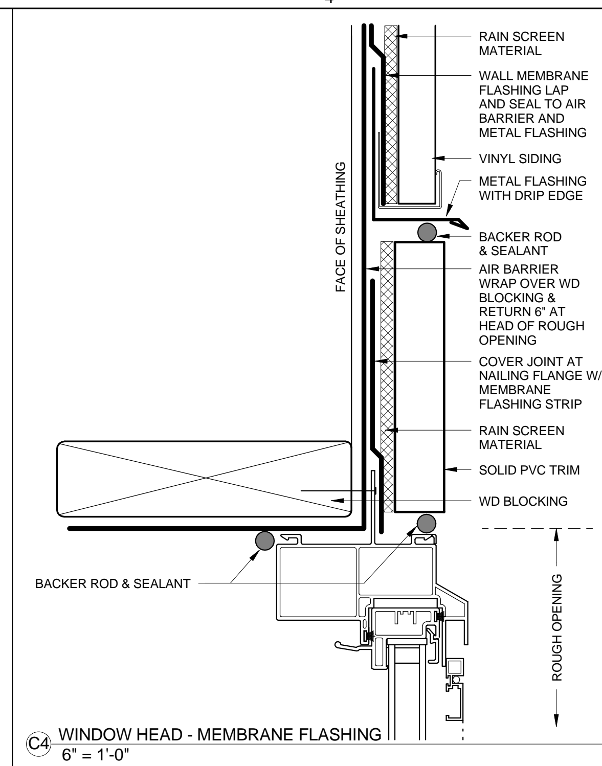
C4 WINDOW HEAD - MEMBRANE FLASHING 6" = 1'-0"
