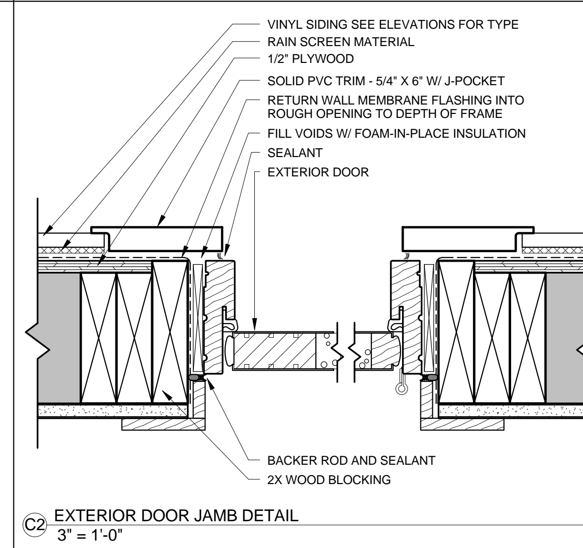
C2 EXTERIOR DOOR JAMB DETAIL 3" = 1'-0"
