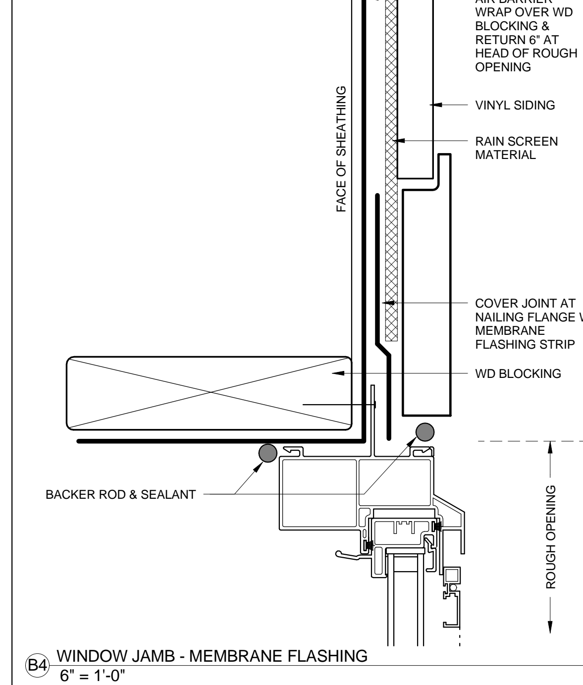
B4 WINDOW JAMB - MEMBRANE FLASHING 6" = 1'-0"
