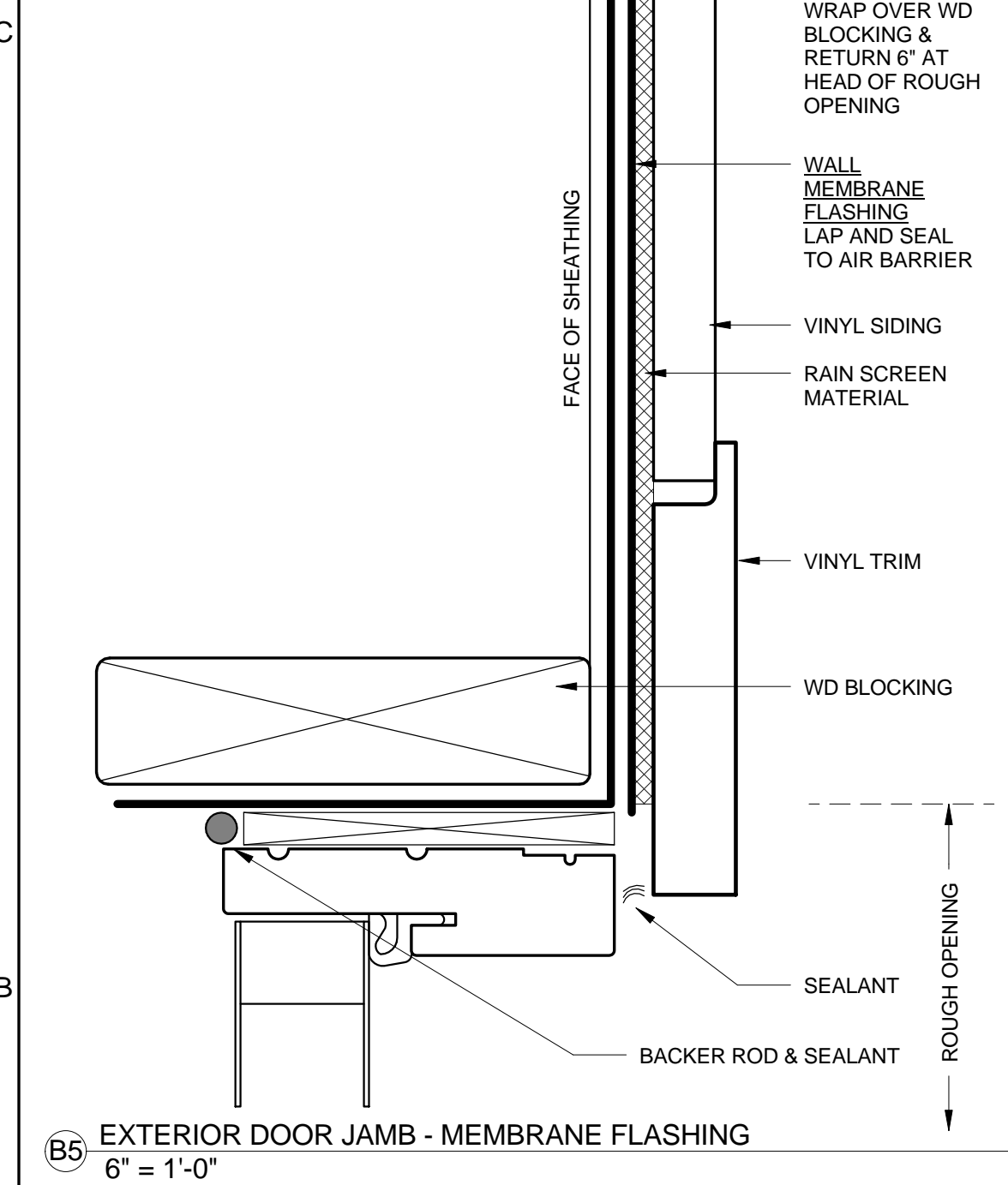
B5 EXTERIOR DOOR JAMB - MEMBRANE FLASHING 6" = 1'-0"
