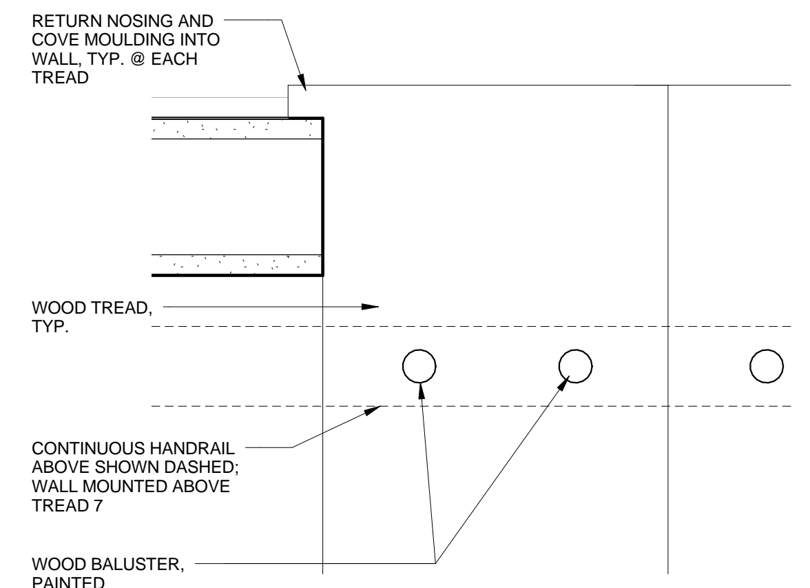
B2 WOOD TREAD DETAIL 3" = 1'-0"
