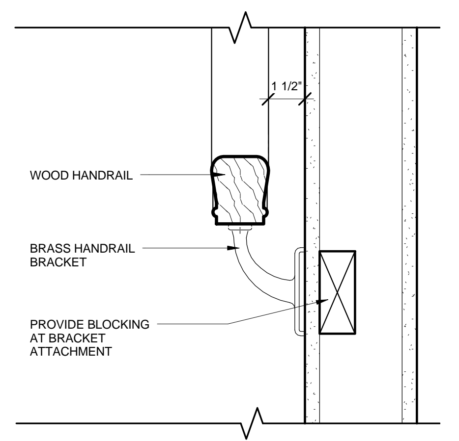
C2 HANDRAIL @ WALL DETAIL 3" = 1'-0"
