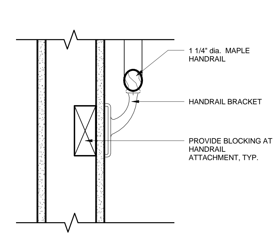
D1 WOOD HANDRAIL DETAIL 3" = 1'-0"
