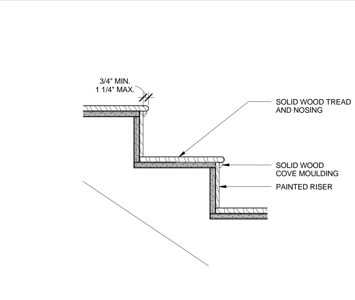
A2 WOOD STAIR DETAIL 1 1/2" = 1'-0"
