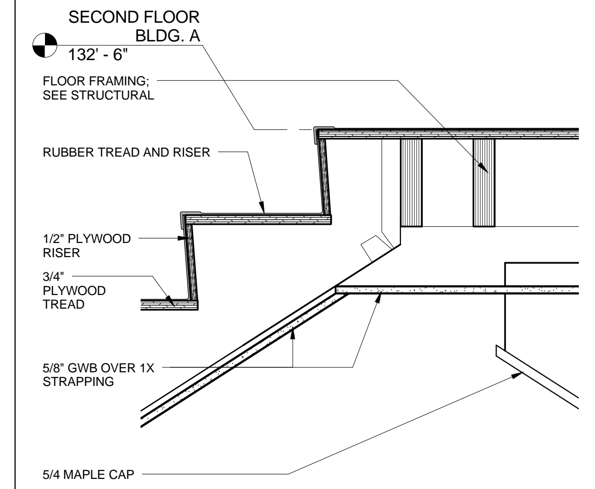
C1 TOP OF STAIR DETAIL 1 1/2" = 1'-0"
