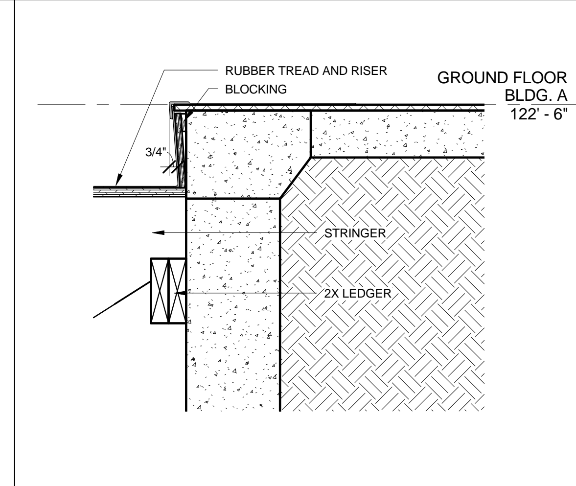
A1 STAIR @ CONCRETE SLAB 1 1/2" = 1'-0"
