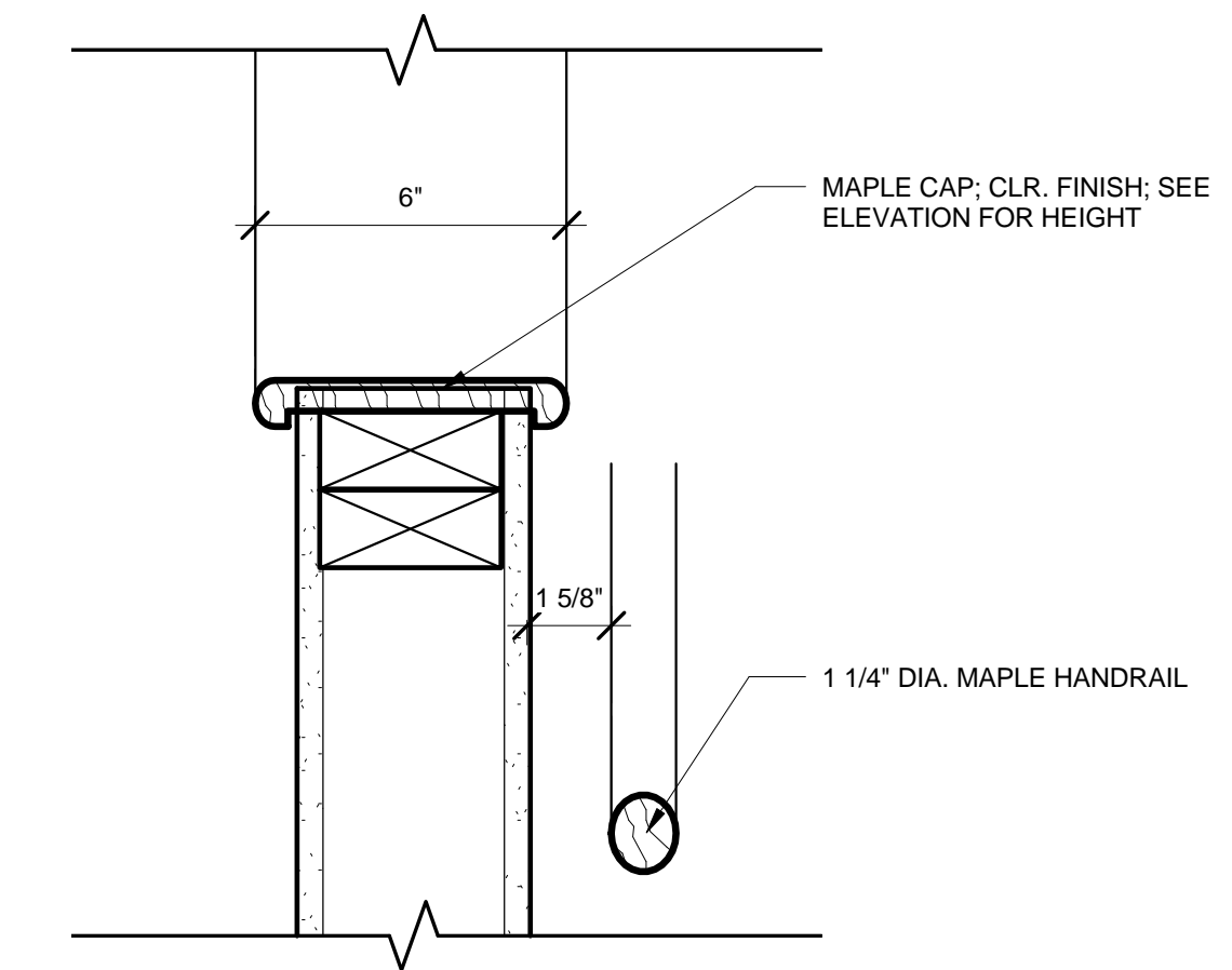
D2 PARTIAL HEIGHT WALL CAP 3" = 1'-0"
