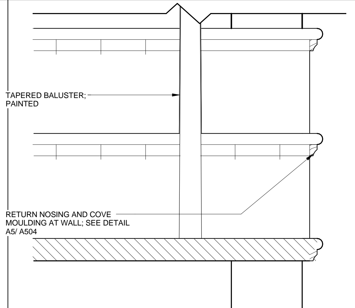
A3 HANDRAIL W/ BALUSTER DETAIL 3" = 1'-0"
