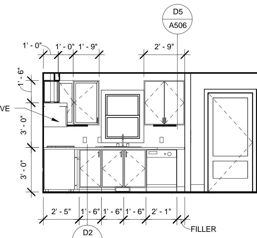
13 TYPICAL KITCHEN - 3BR UNIT 1/4" = 1'-0"
