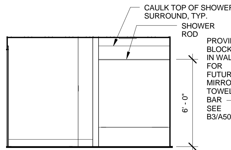
12 TYPICAL BATH - 3BR UNIT 1/4" = 1'-0"
