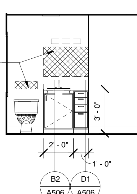
24 BATH - 3BR UNIT 1/4" = 1'-0"
