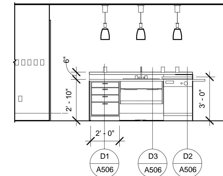
2 TYPE A KITCHEN ISLAND- A101- WEST- BLDG A 2BR UNIT 1/4" = 1'-0"
