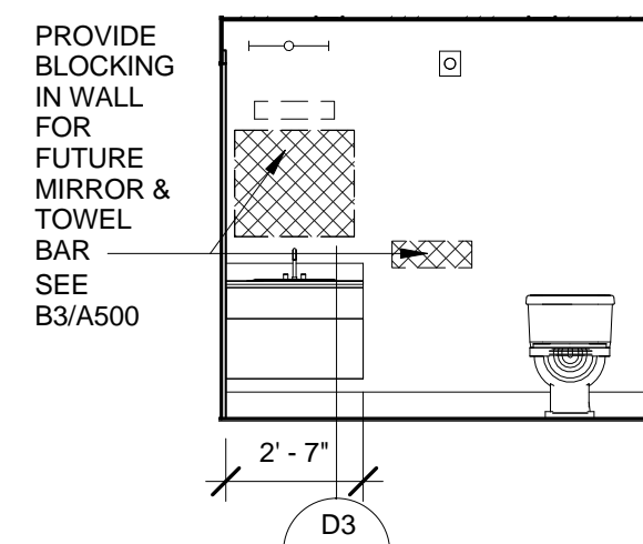
10 TYPICAL BATH - 2BR UNIT 1/4" = 1'-0"
