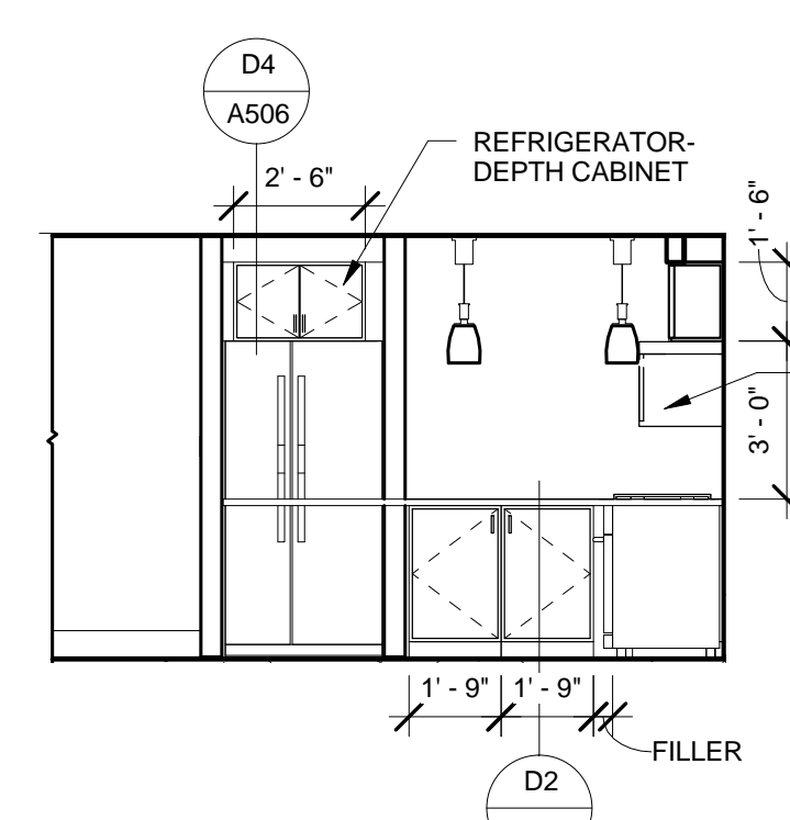
15 KITCHEN - 3BR UNIT 1/4" = 1'-0"
