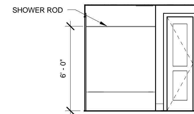
9 TYPICAL BATH - 2BR UNIT 1/4" = 1'-0"
