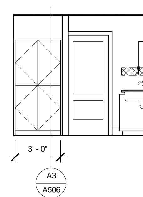
21 BATH - 2BR UNIT 1/4" = 1'-0"
