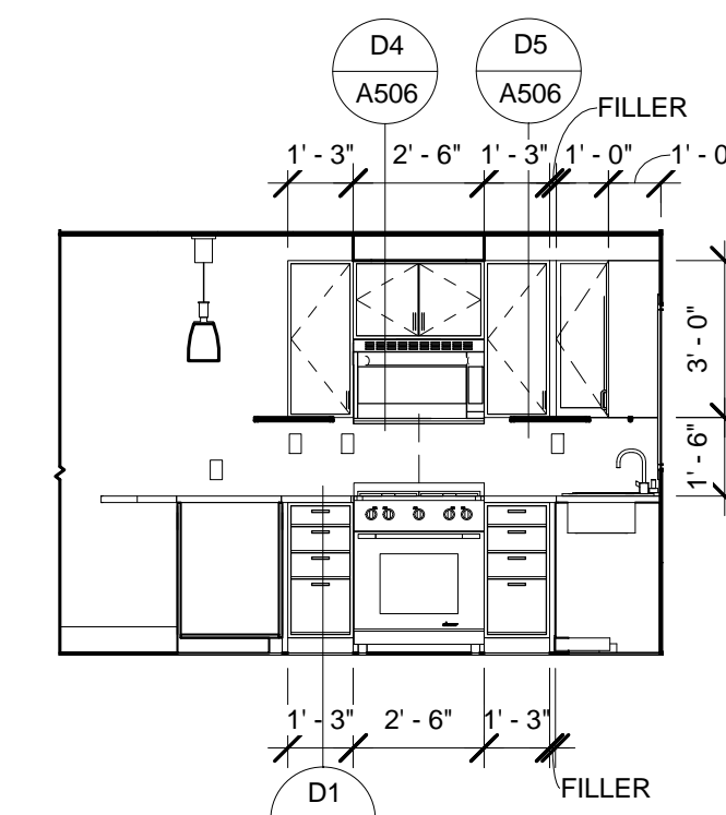
14 TYPICAL KITCHEN - 3BR UNIT 1/4" = 1'-0"
