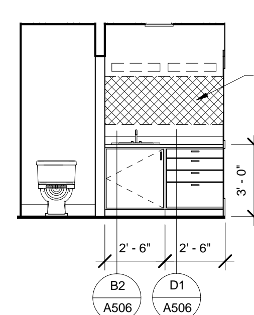
22 BATH - 3BR UNIT 1/4" = 1'-0"
