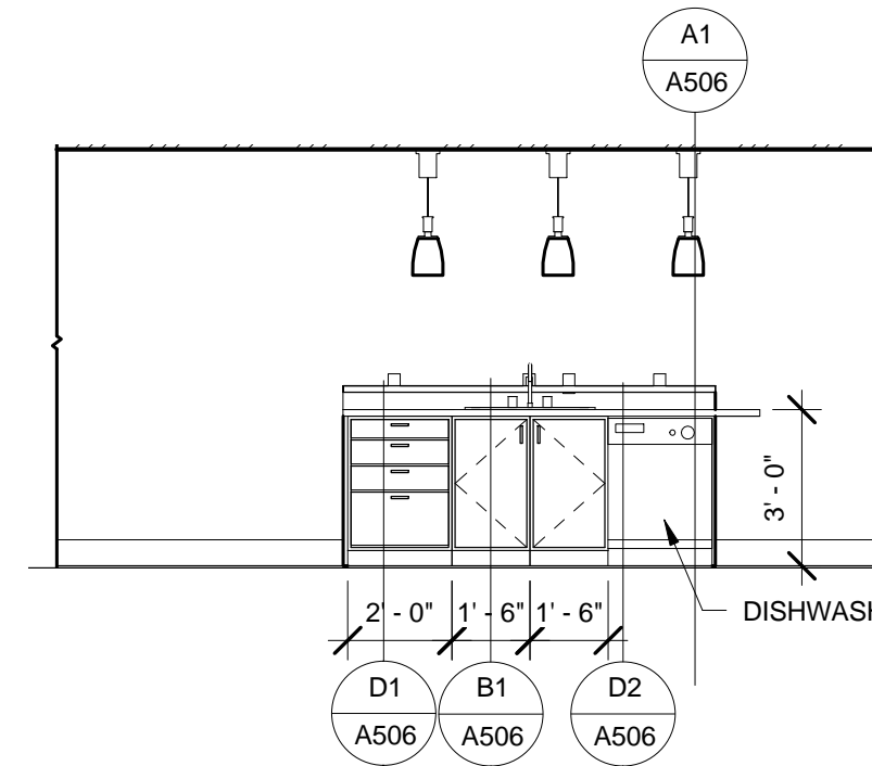
3 KITCHEN ISLAND - 2BR UNIT 1/4" = 1'-0"
