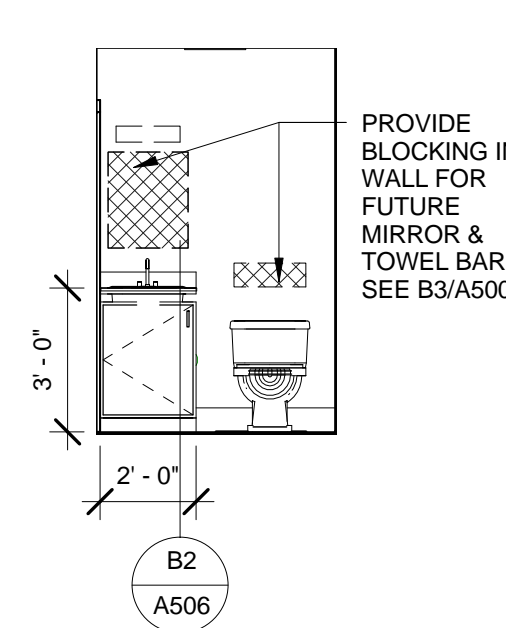
20 POWDER - 2BR UNIT 1/4" = 1'-0"
