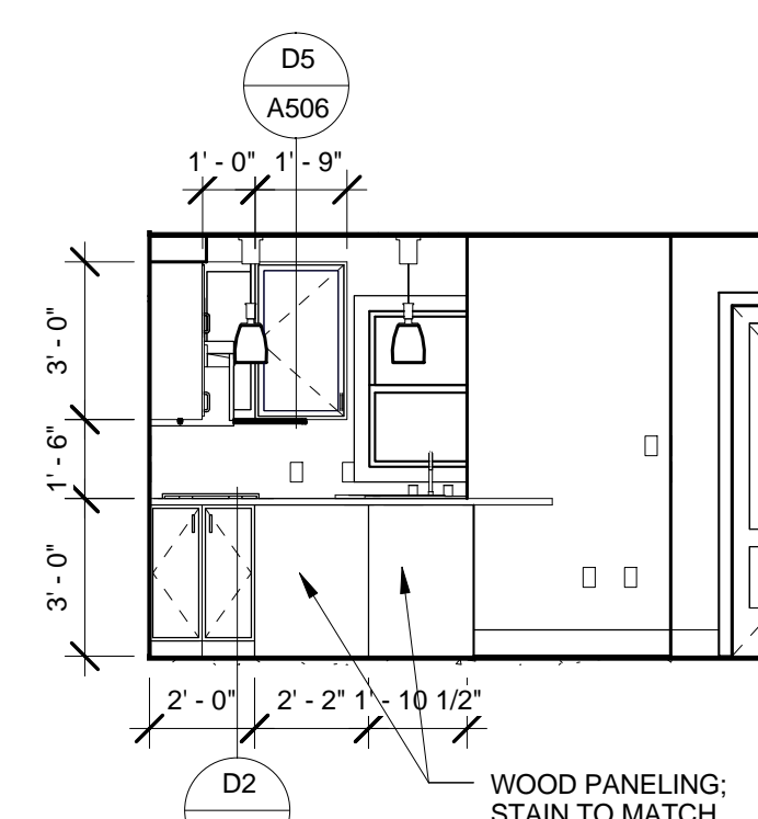
16 KITCHEN/LIVING - 3BR UNIT 1/4" = 1'-0"
