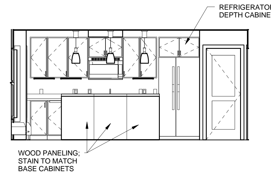
4 KITCHEN ISLAND - 2BR UNIT 1/4" = 1'-0"
