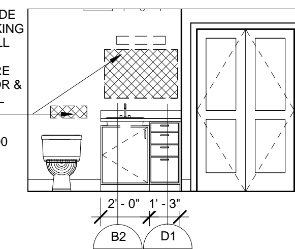
11 TYPICAL BATH - 3BR UNIT 1/4" = 1'-0"
