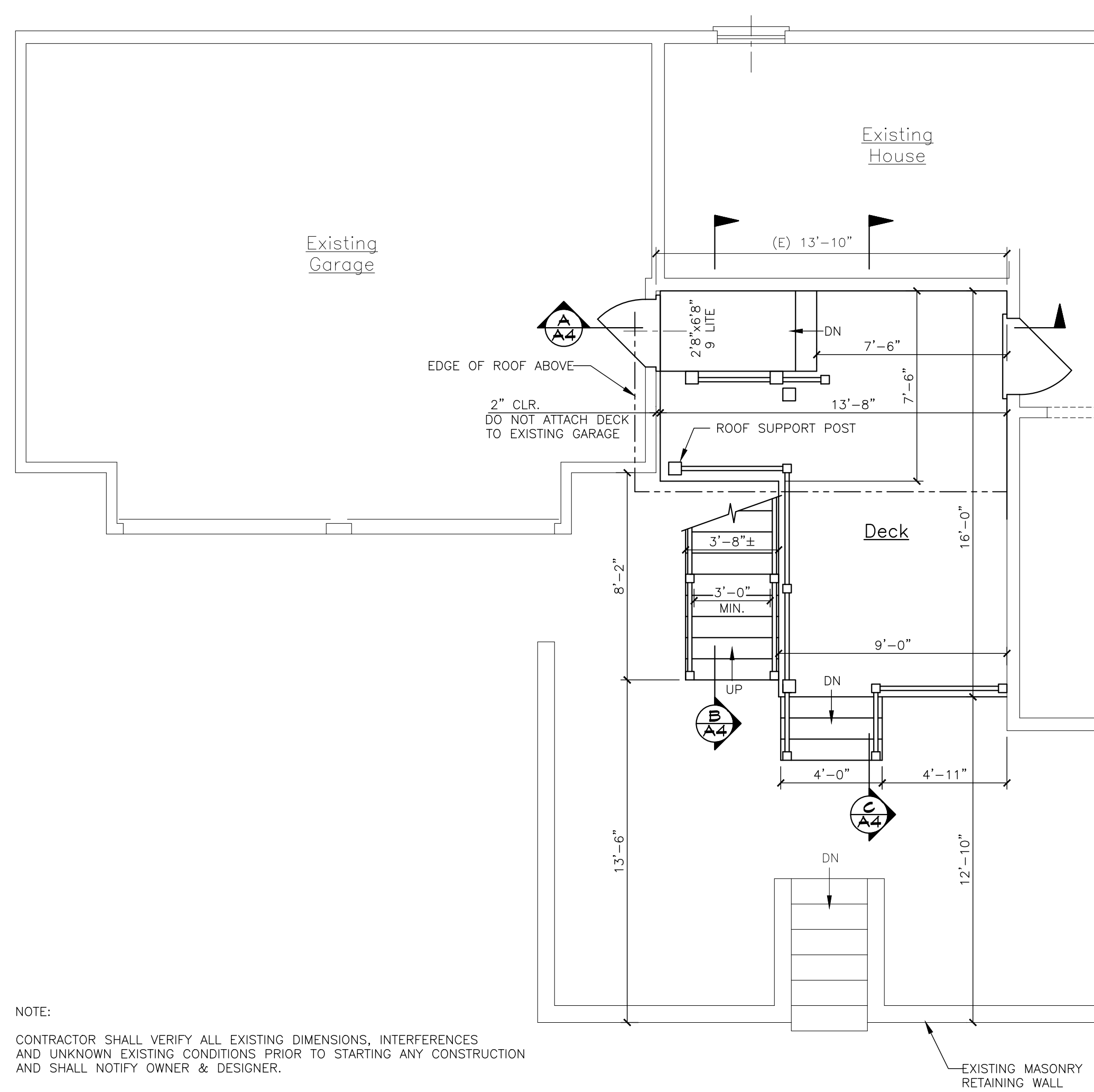
DECK FLOOR PLAN—FIRST FLOOR
