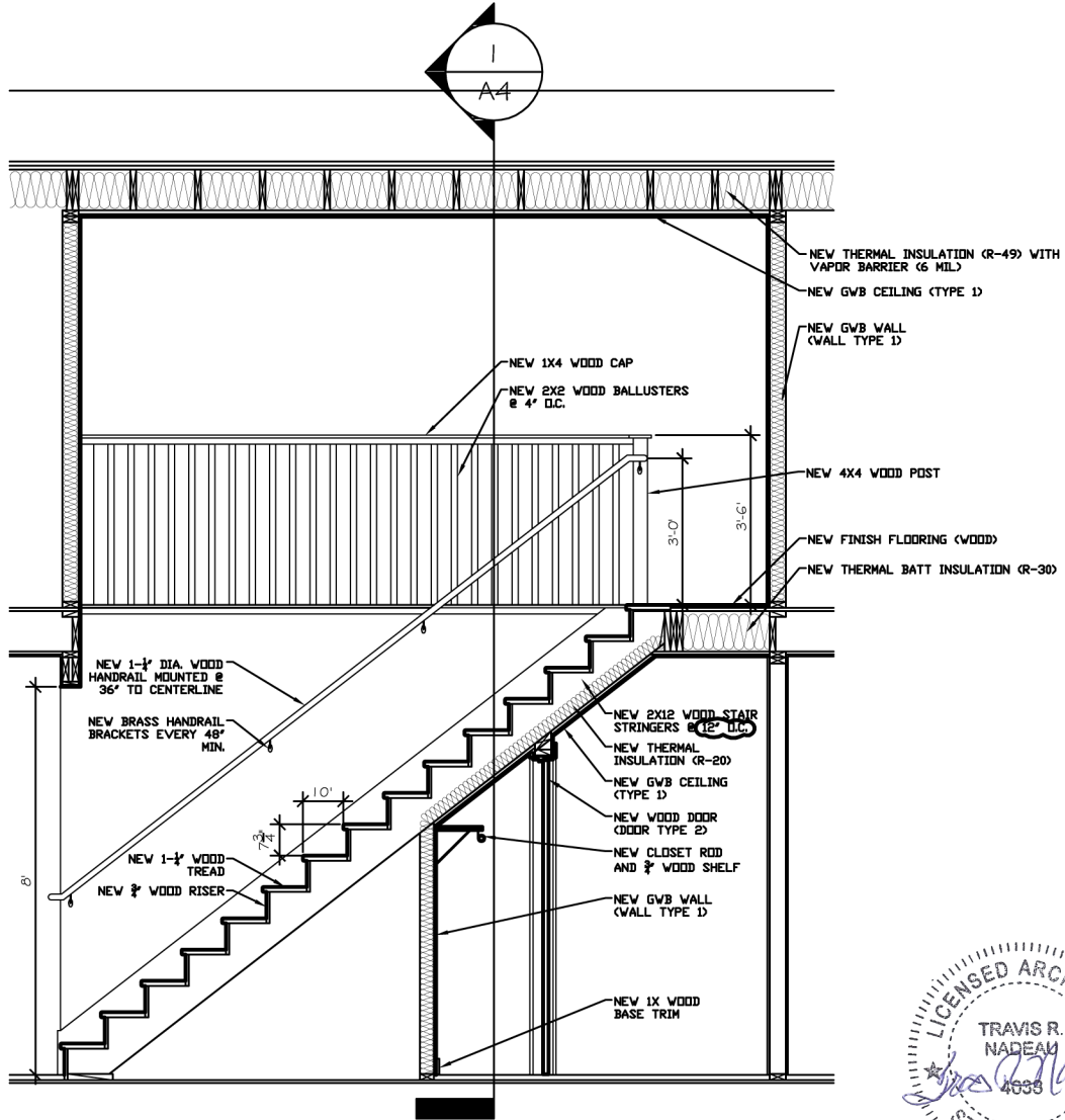
1. STAIR SECTION
