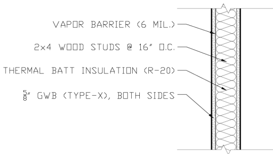
WALL TYPE 1
