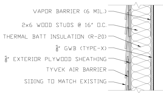
WALL TYPE 2
