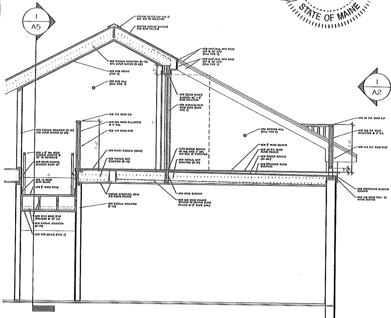
1. BUILDING SECTION
