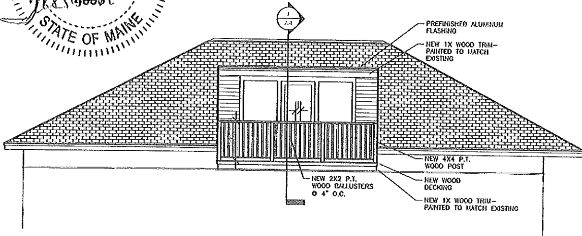
1. PROPOSED EXTERIOR ELEVATION
