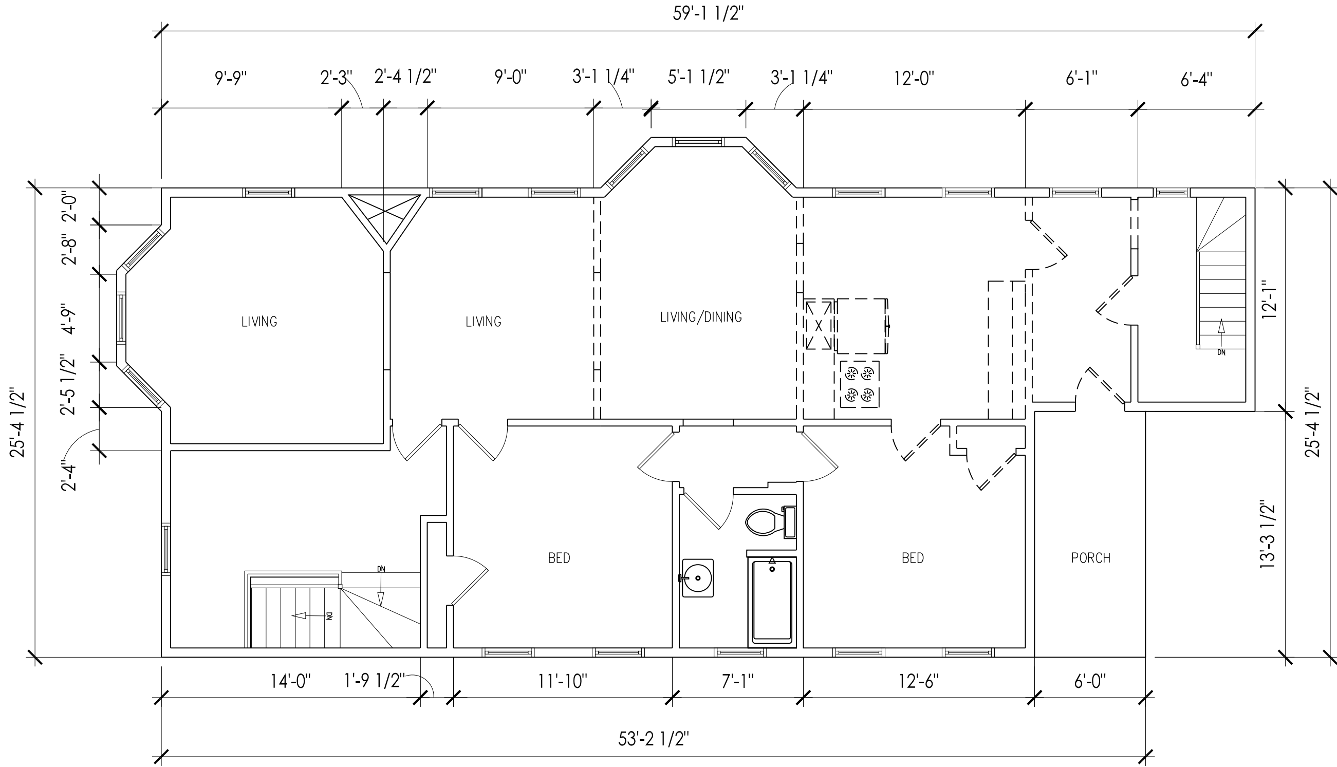
THIRD LEVEL PLAN SCALE 3/16" = 1'-0"
