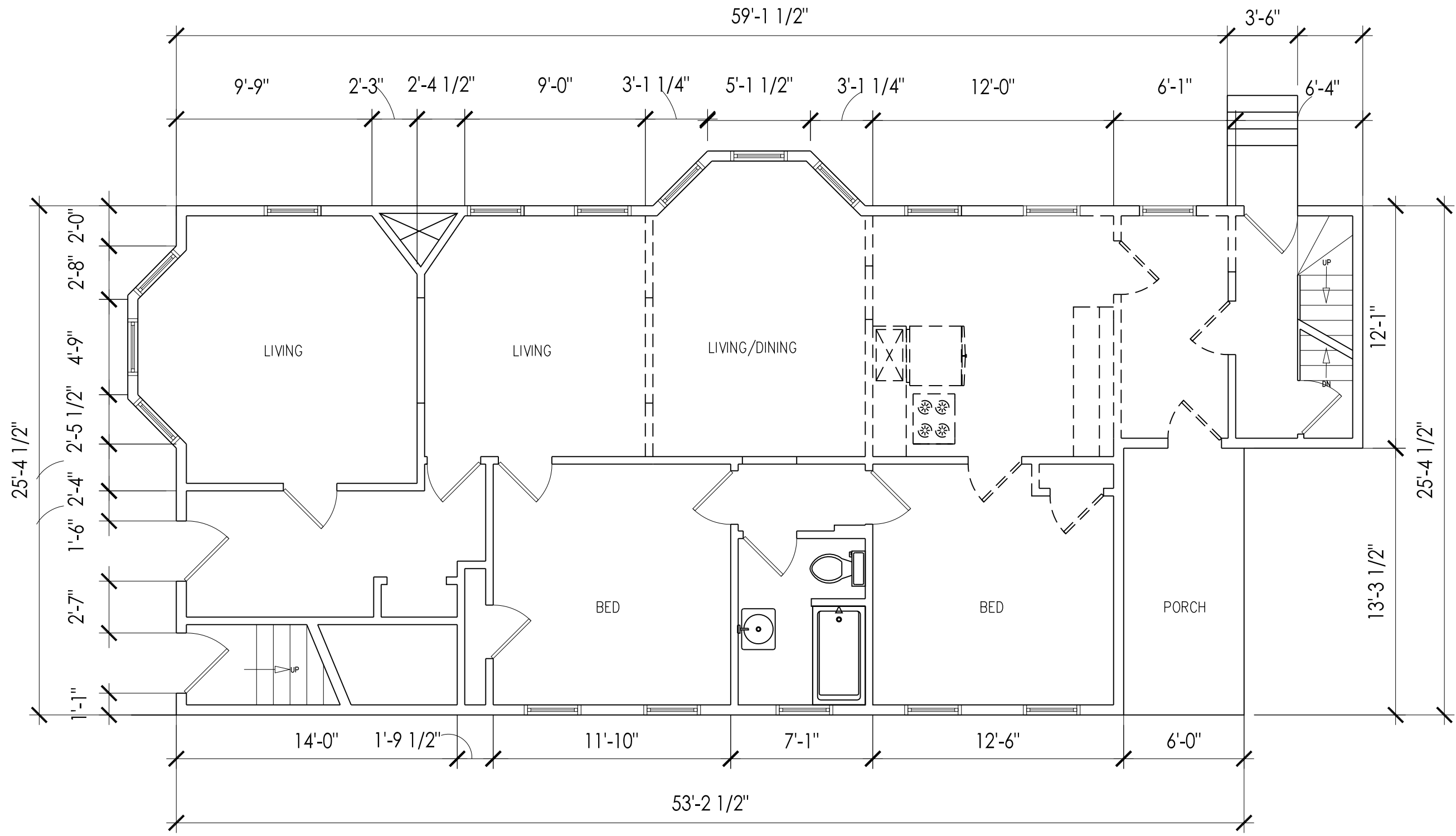
FIRST LEVEL PLAN SCALE 3/16" = 1'-0"
