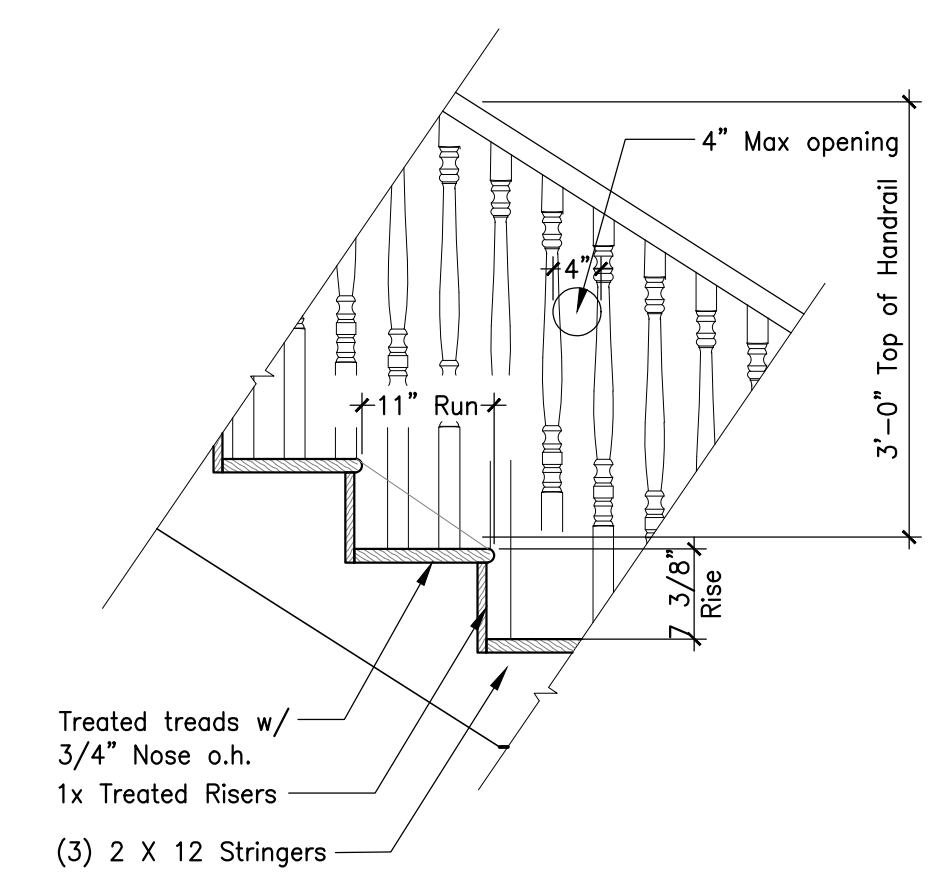
2 Exterior Stair Section & Detail Scale: 3/4" = 1'-0"
