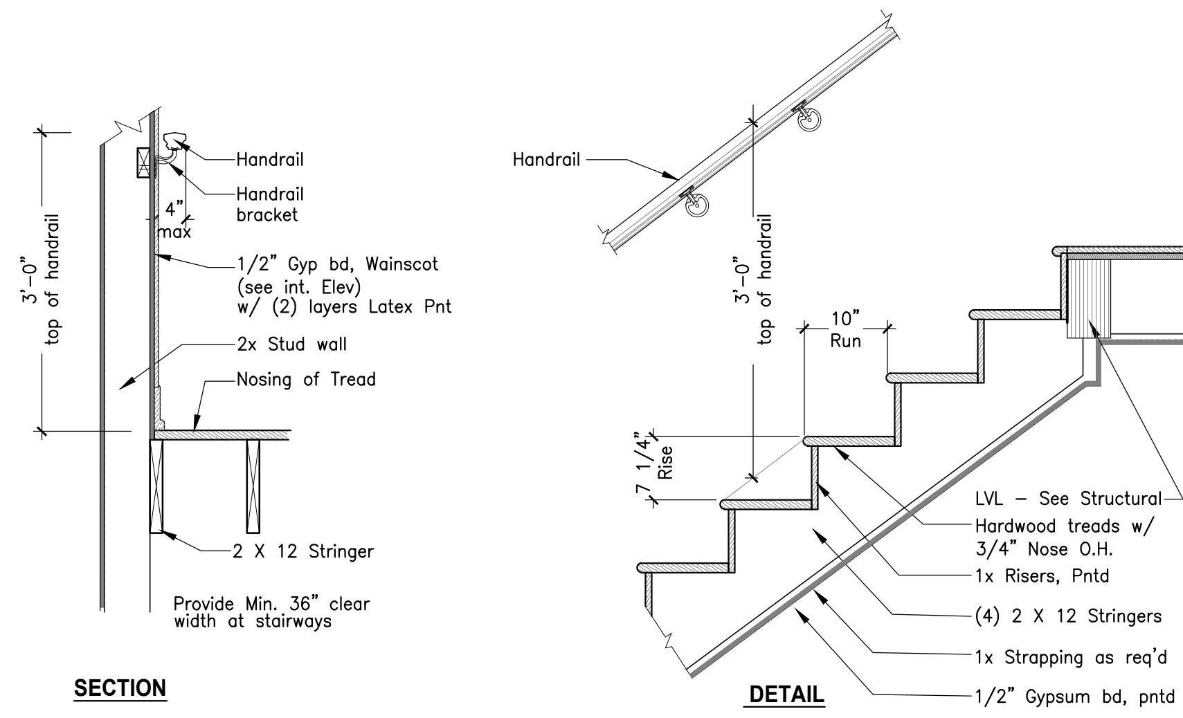
1 New Interior Stair Section & Detail Scale: 3/4" = 1'-0"
