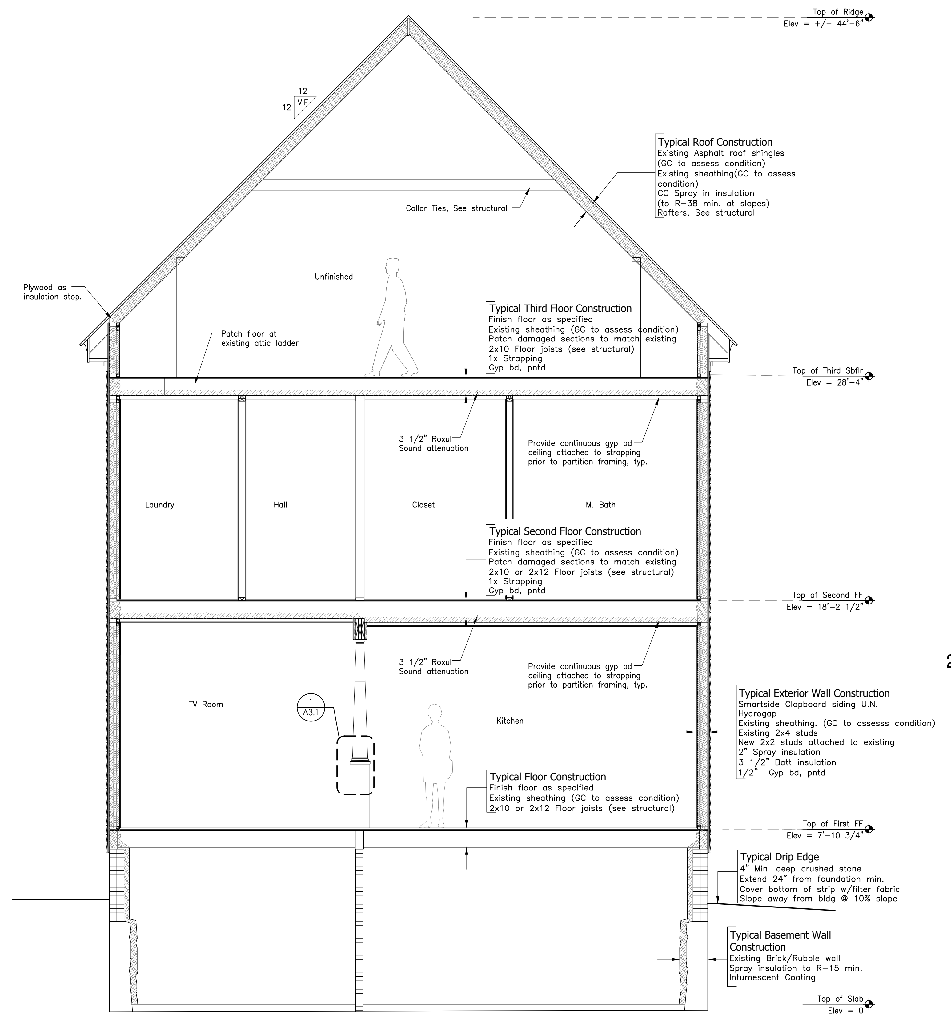
Proposed Building Section
