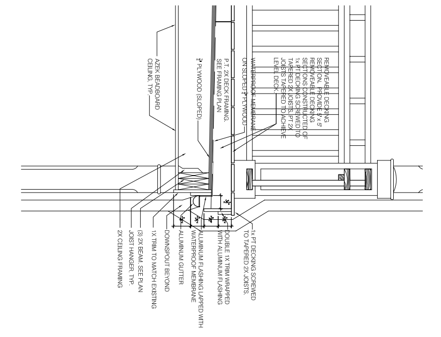
8 SECTION @ THIRD FLOOR DECK SCALE - 1" = 1'-0"
