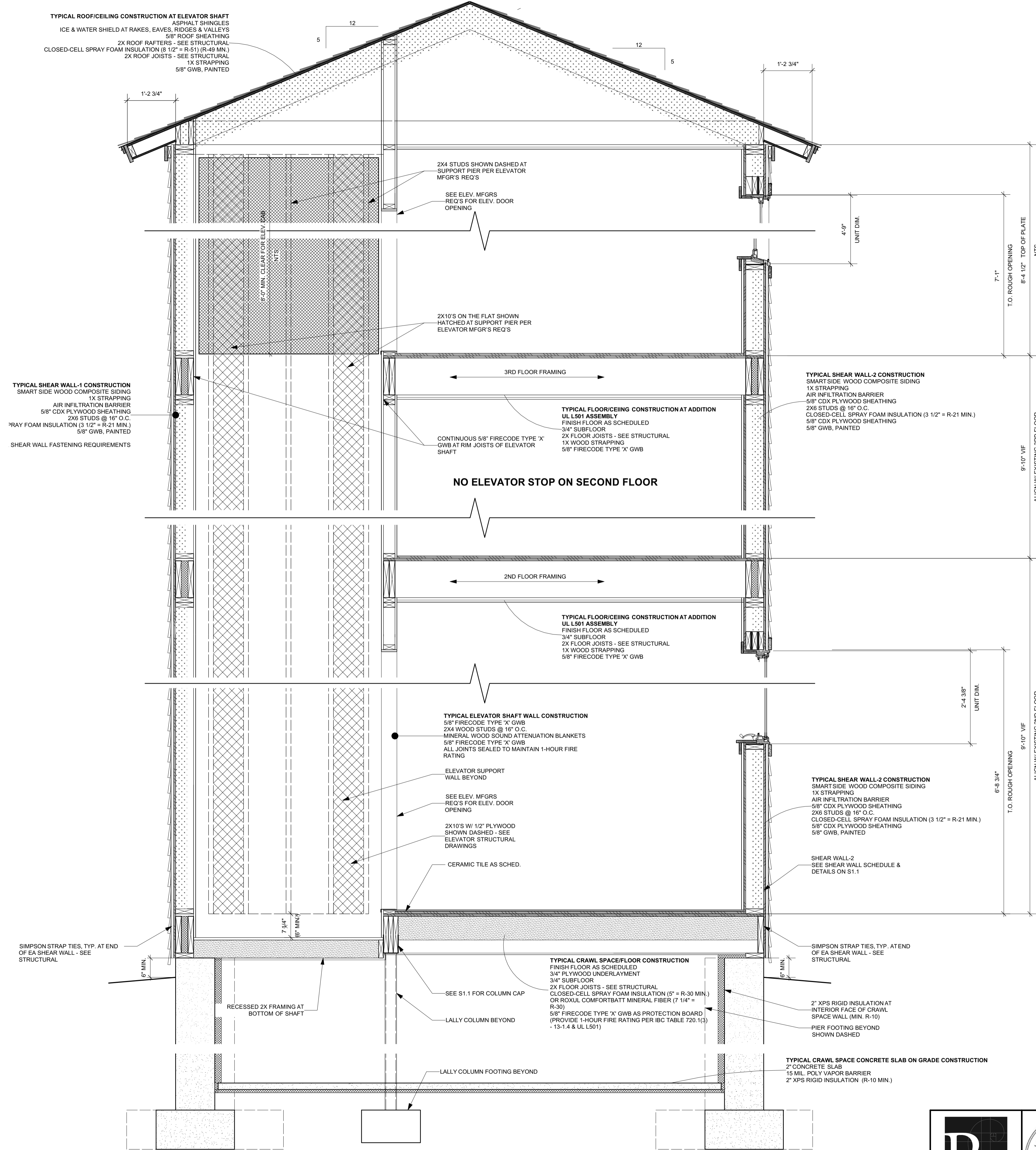
1 WALL SECTION Scale: 3/4" = 1'-0"
