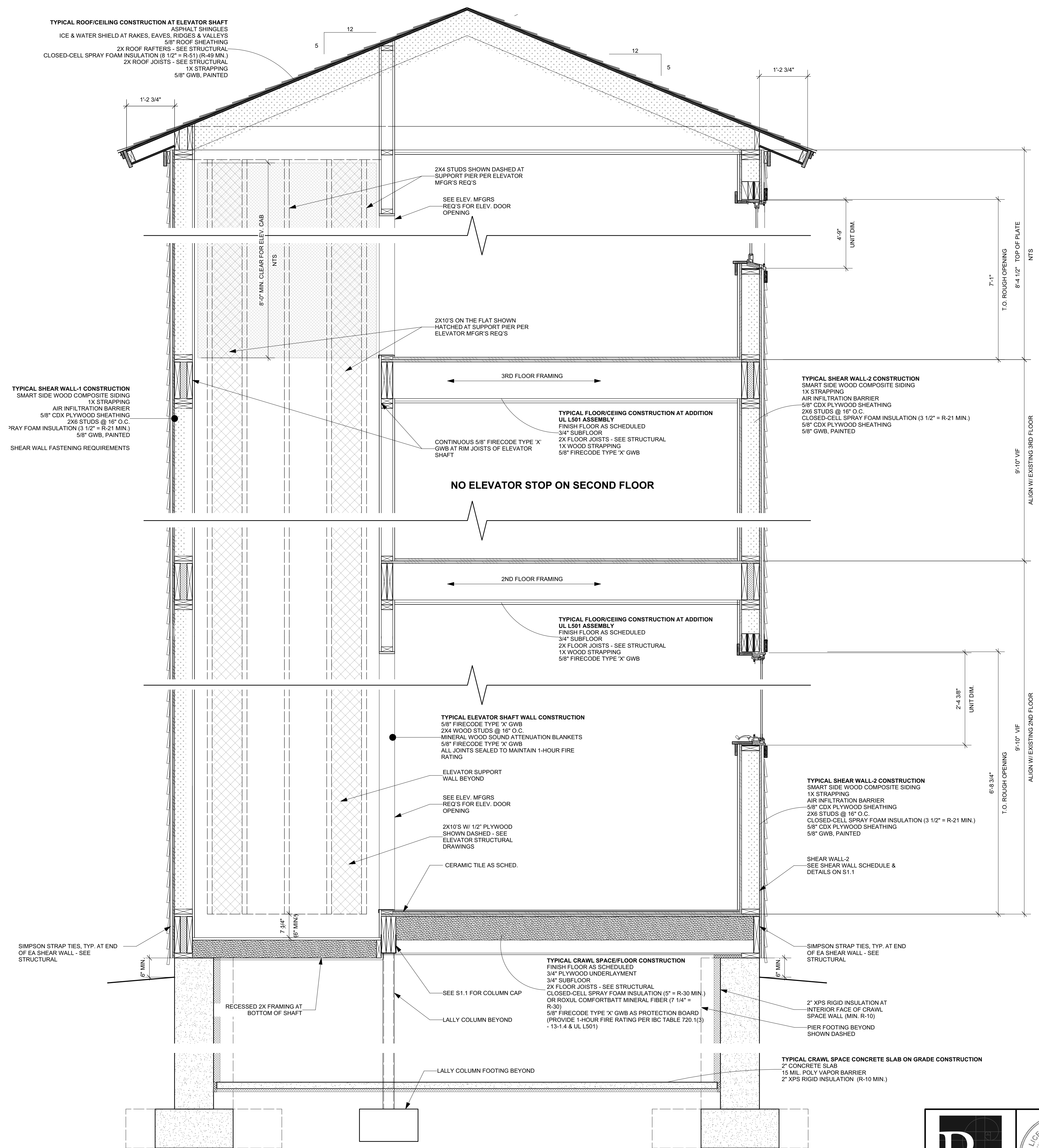
1 WALL SECTION Scale: 3/4" = 1'-0"
