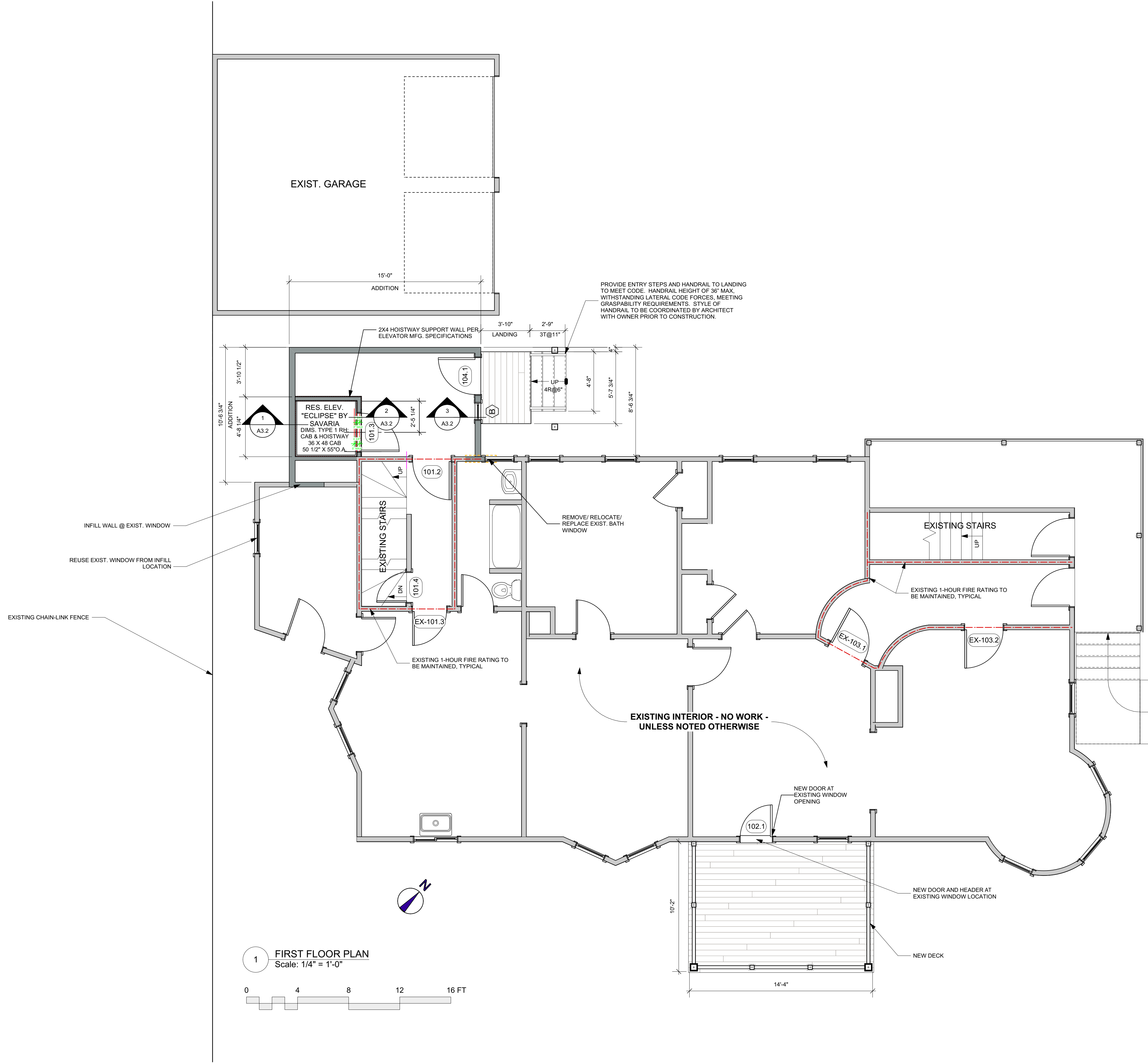
FIRST FLOOR KEY PLAN
