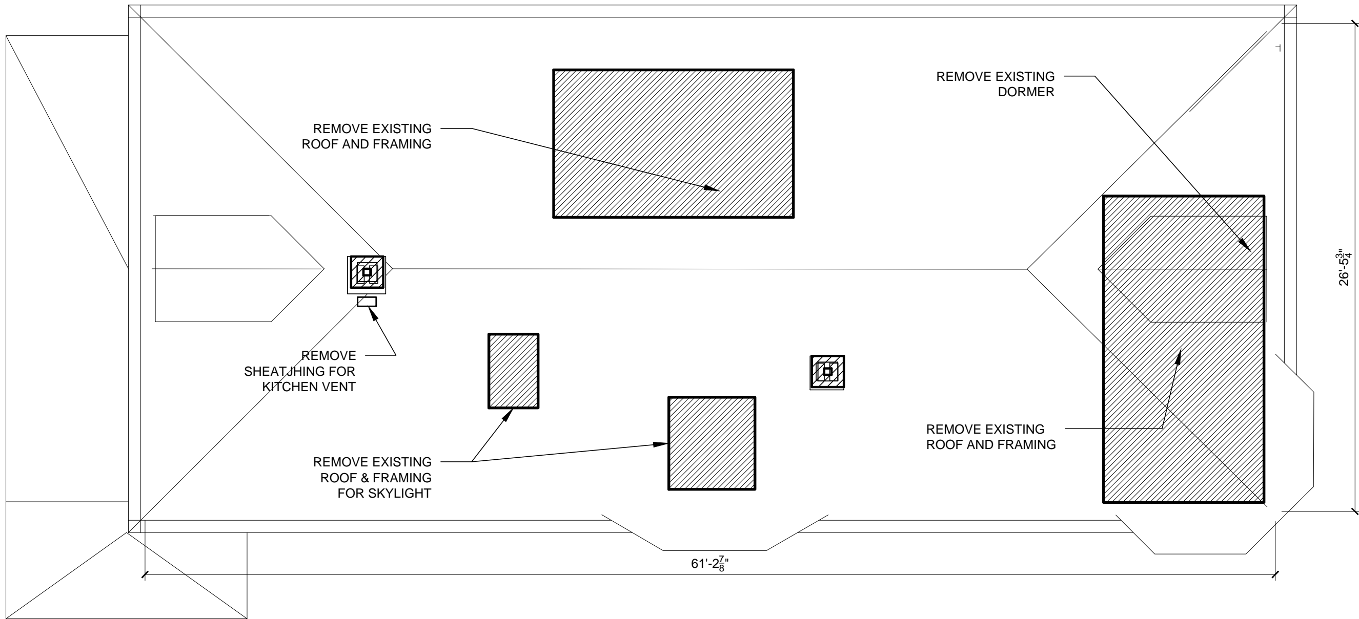
1 ROOF DEMO PLAN 3/16" = 1'-0"
