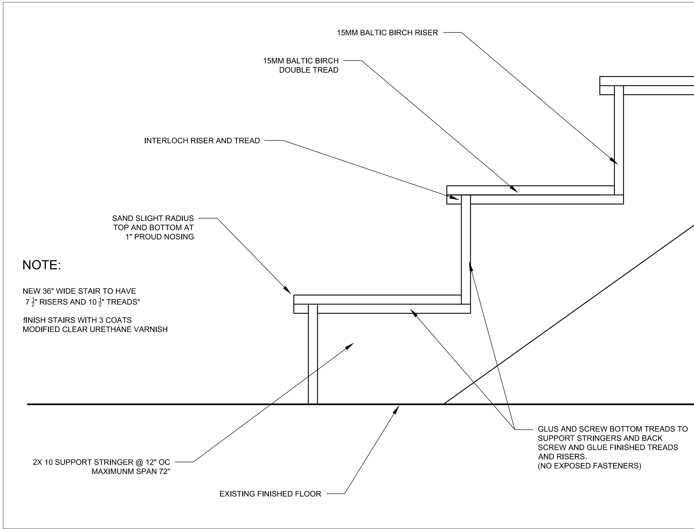
STAIR SECTION 3" = 1'-0"
