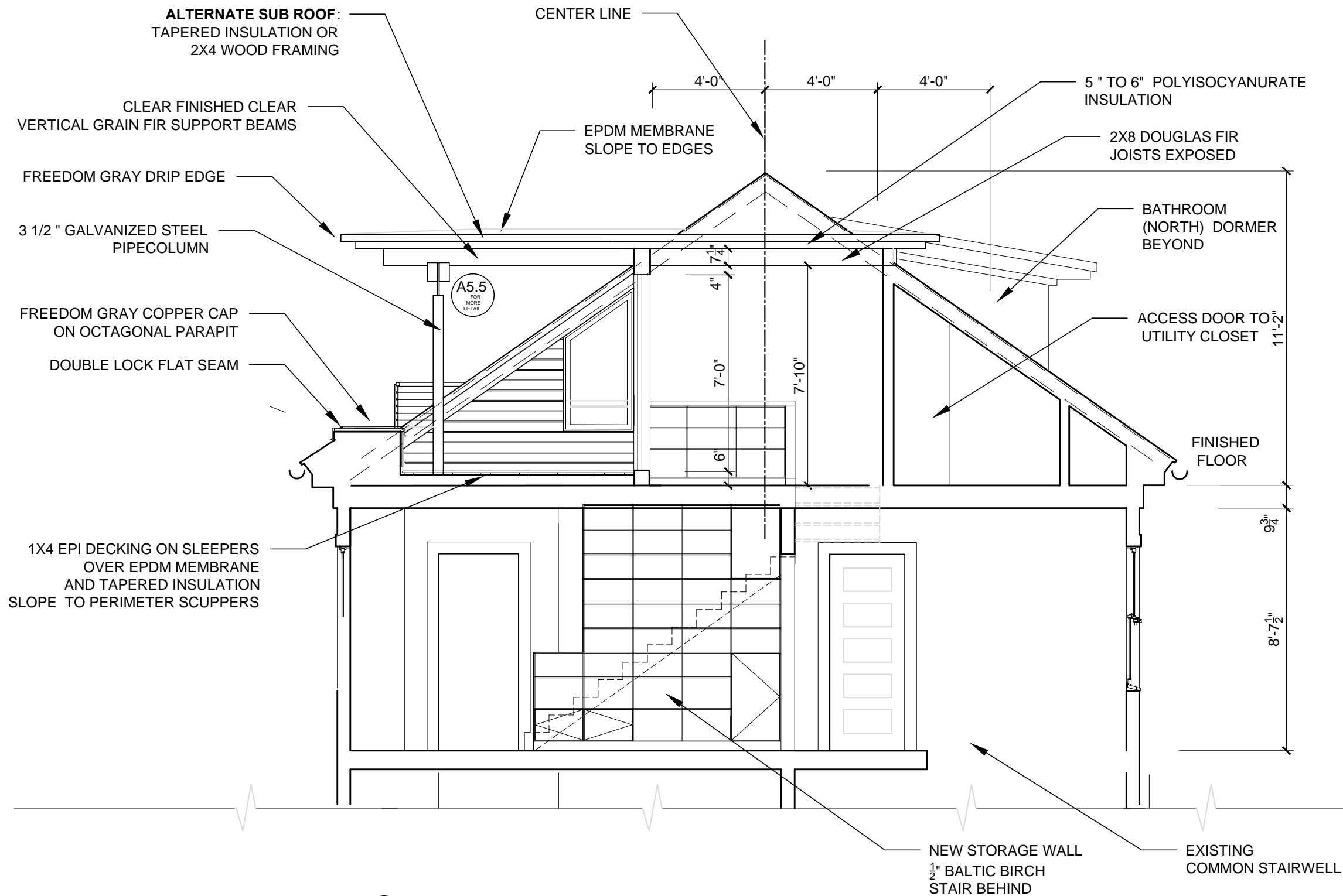
1 CROSS SECTION @ PORCH LOOKING WEST 1/8" = 1'-0"
