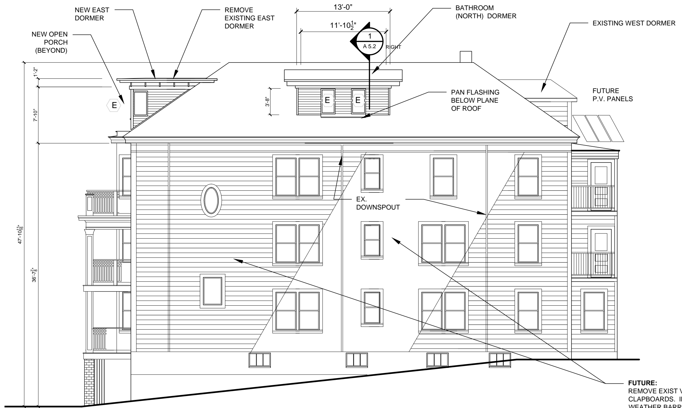
1 NORTH ELEVATION 1/8" = 1'-0"
