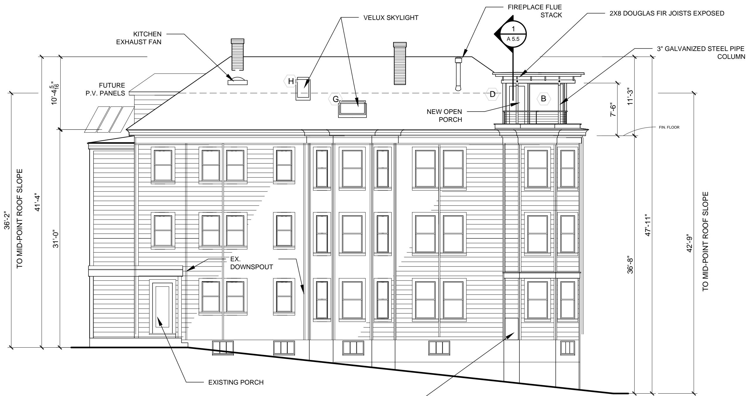
1 SOUTH ELEVATION 1/8" = 1'-0"
