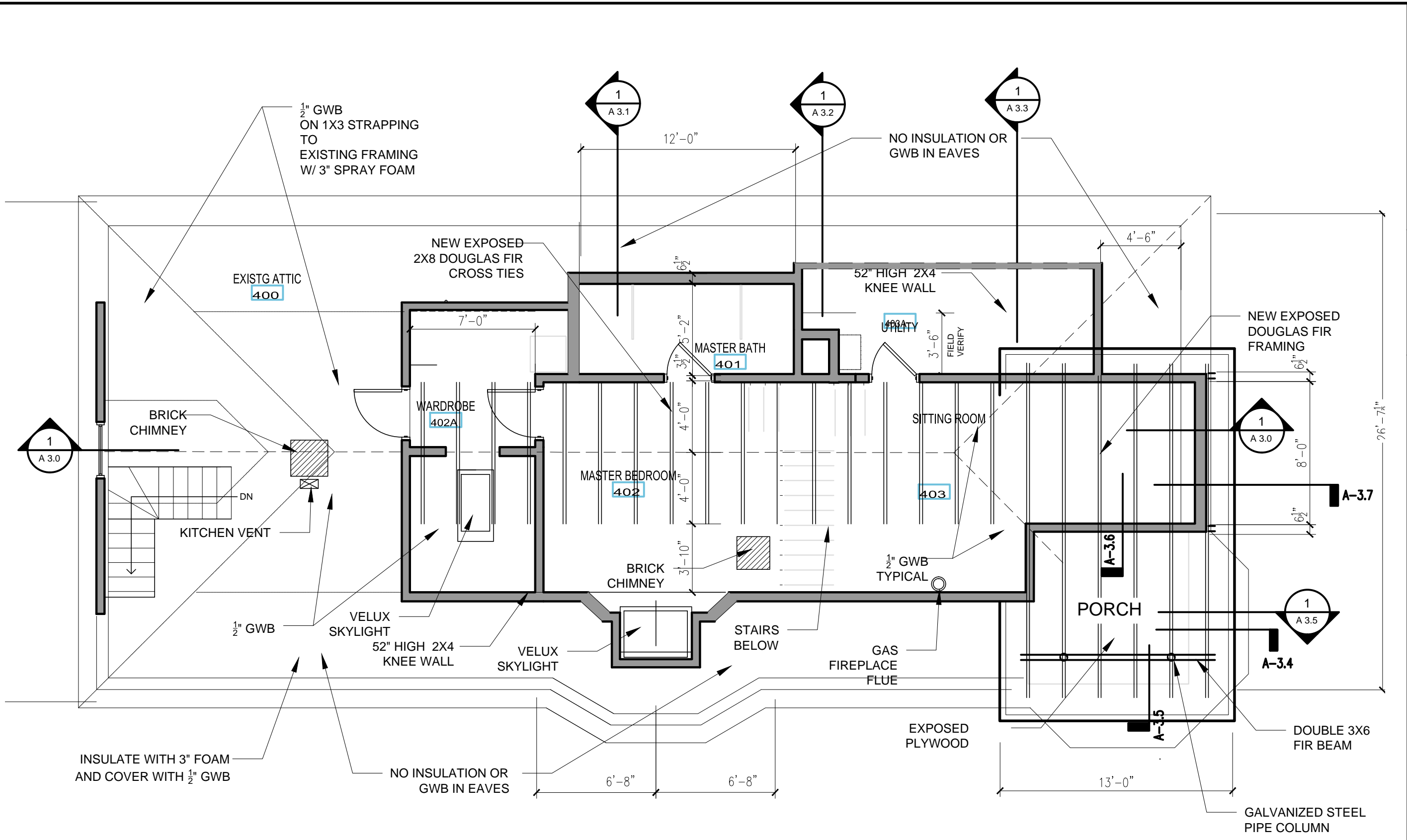
1 ATTIC FLOOR CEILING PLAN 3/16" = 1'-0"
