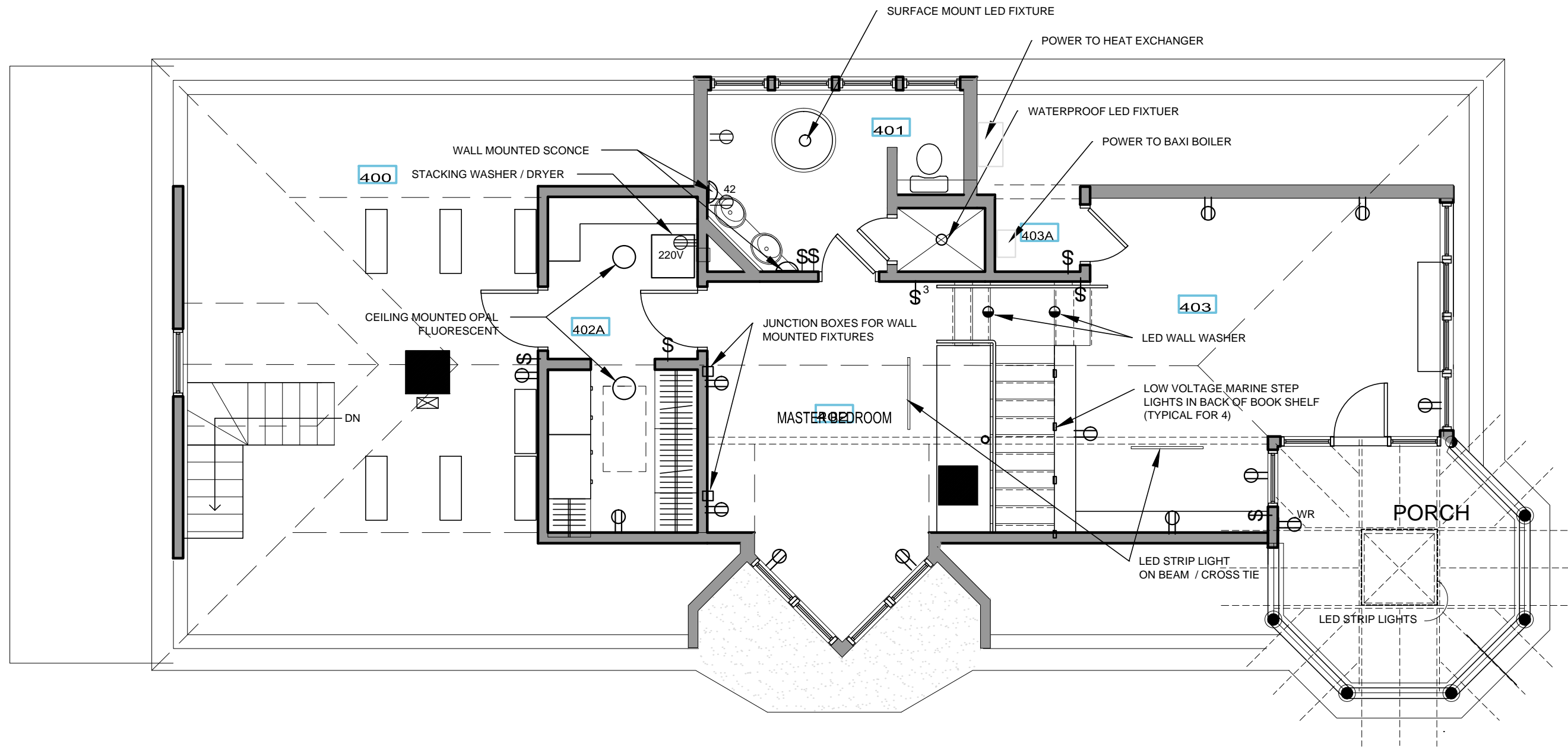
1 POWER & LIGHTING PLAN - ATTIC 3/16" = 1'-0"
