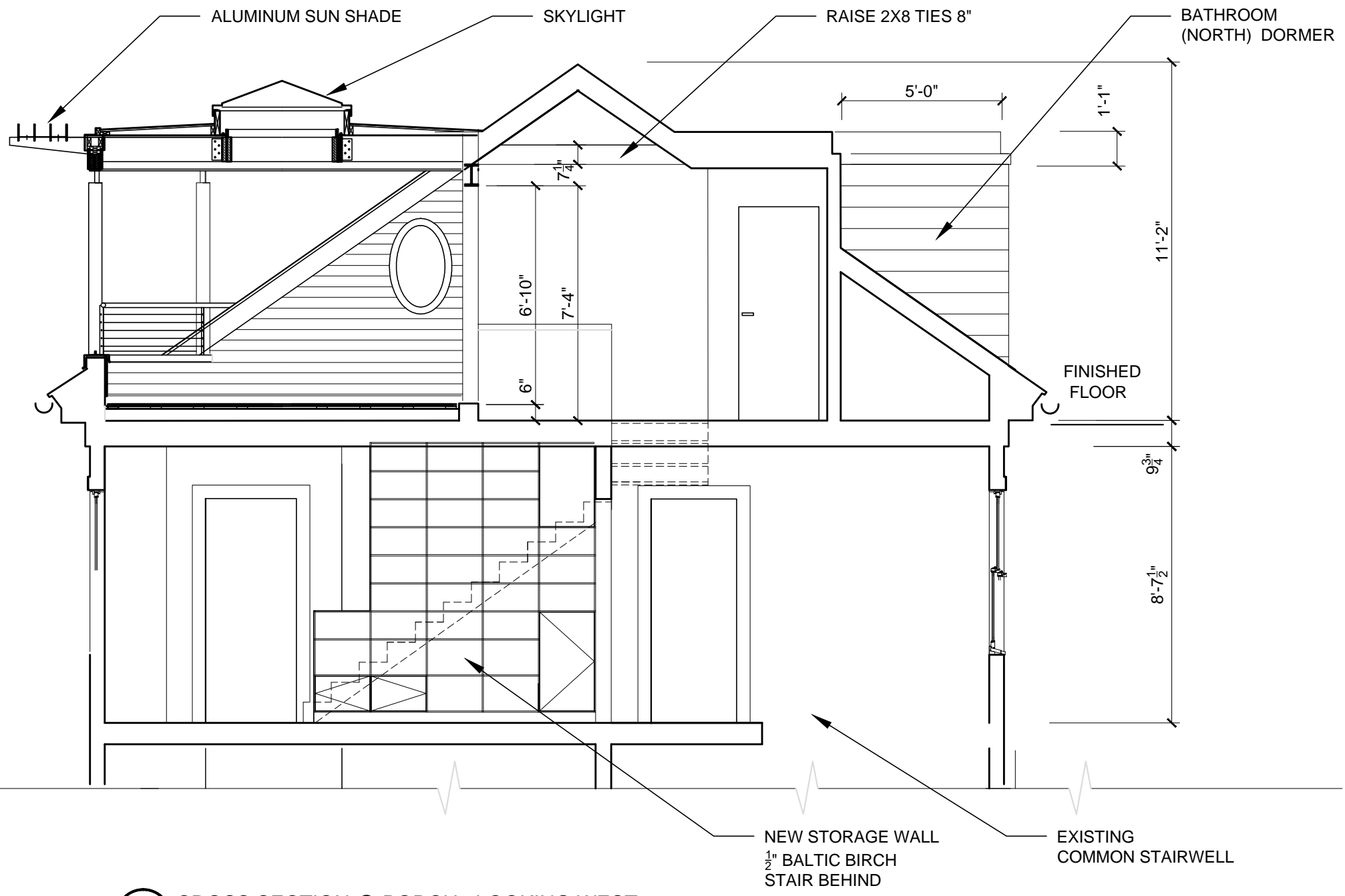
1 CROSS SECTION @ PORCH LOOKING WEST 1/8" = 1'-0"
