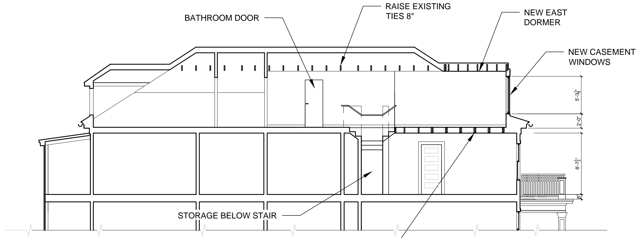
1 LONGITUDINAL SECTION LOOKING NORTH 1/8" = 1'-0"
