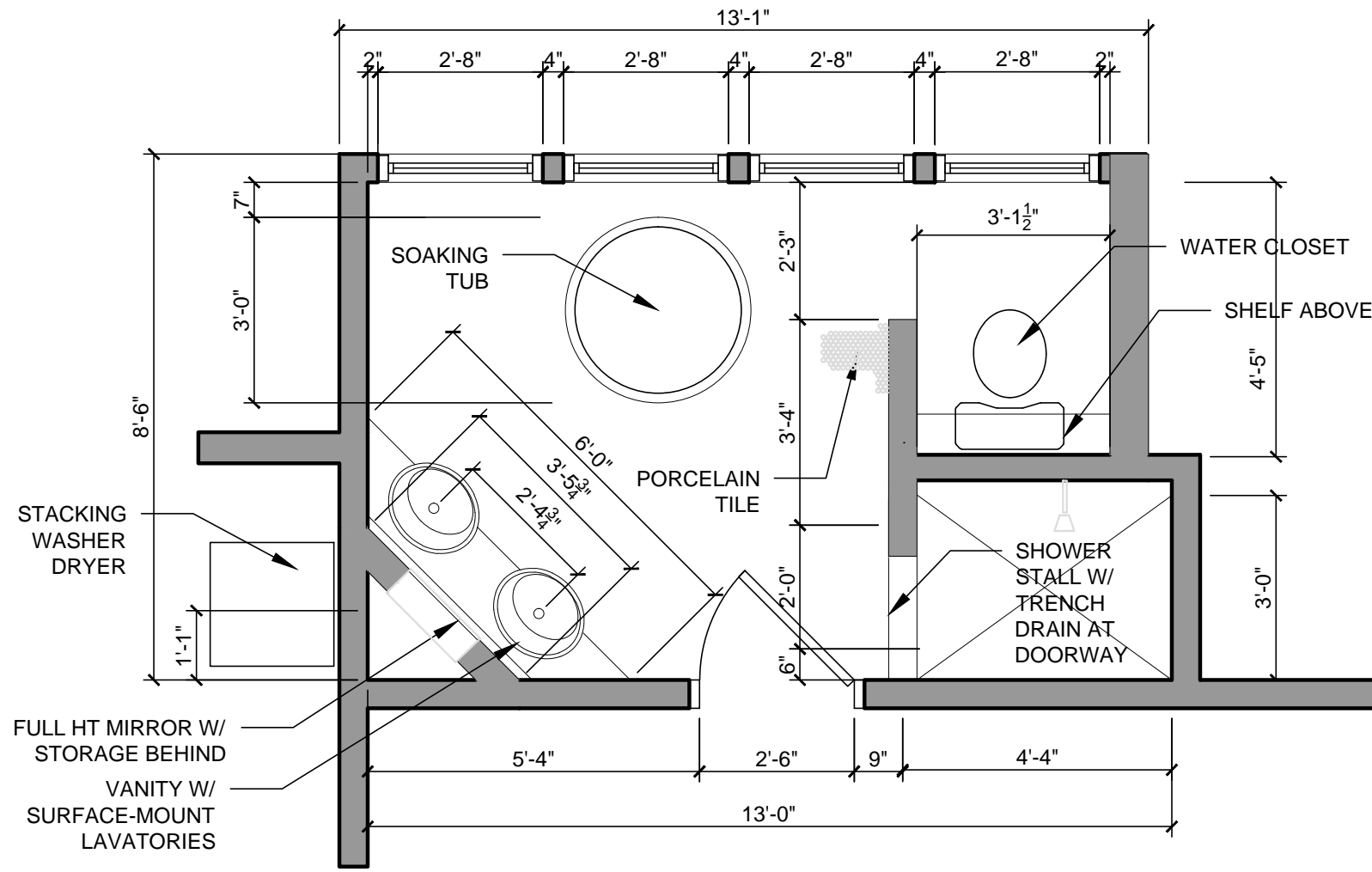
1 BATH - DETAIL PLAN NEW NORTH DORMER 3/8" = 1'-0"
