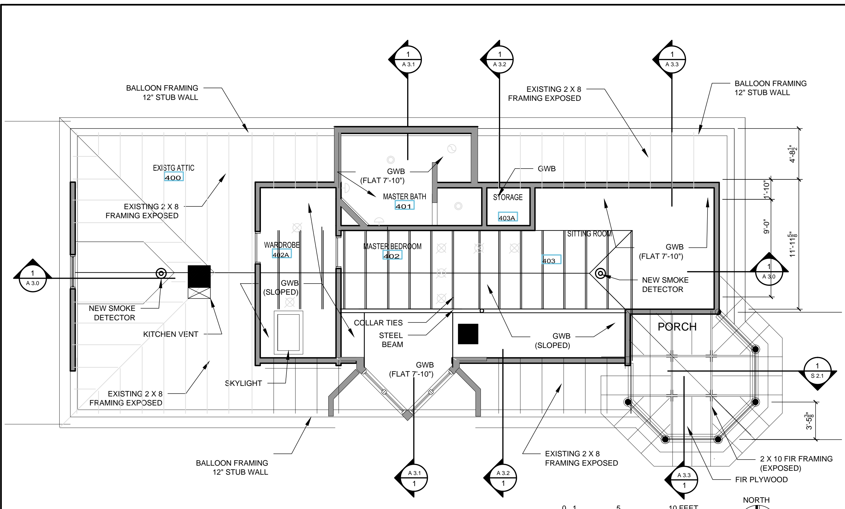
1 ATTIC FLOOR REFLECTED CEILING PLAN 1/8" = 1'-0"
