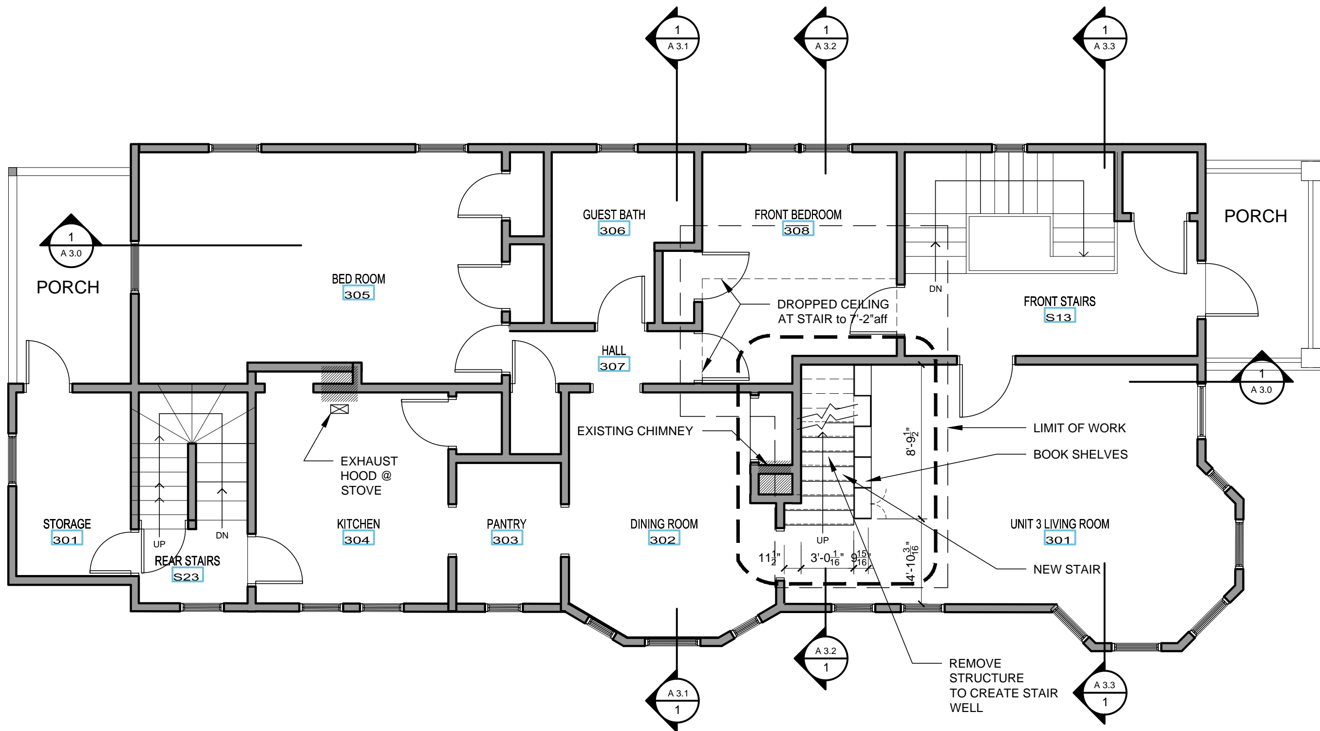
1 PROPOSED THIRD FLOOR 3/16" = 1'-0"
