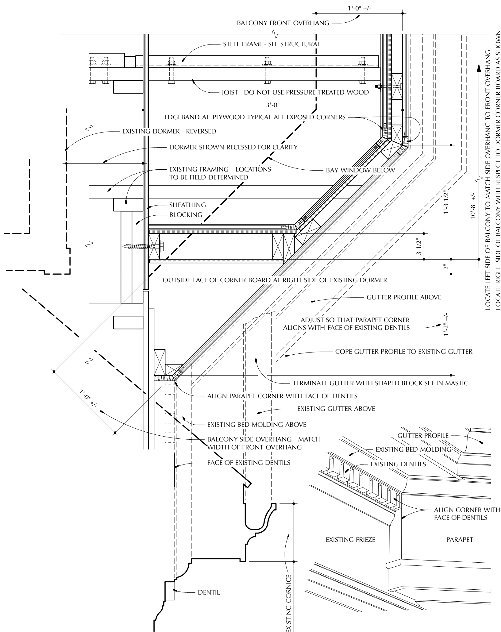
1 PLAN DETAIL AT PARAPET Scale: 1 1/2" = 1'-0"
