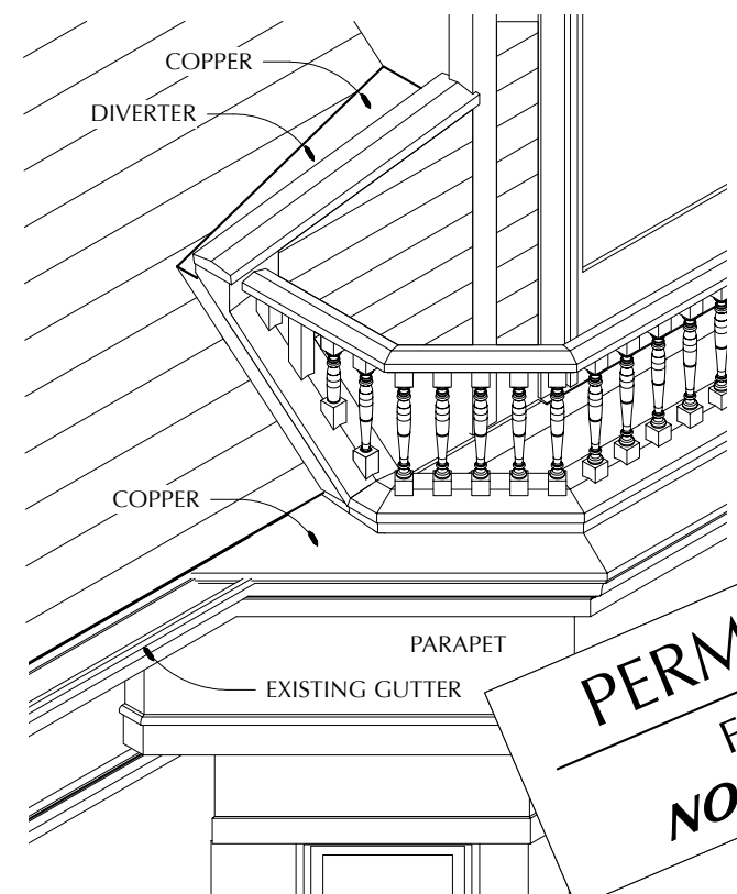
5 CORNICE & DIVERTER Not To Scale
