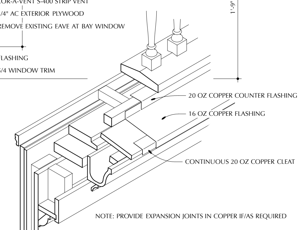
6 PARAPET CORNICE DETAIL Not To Scale
