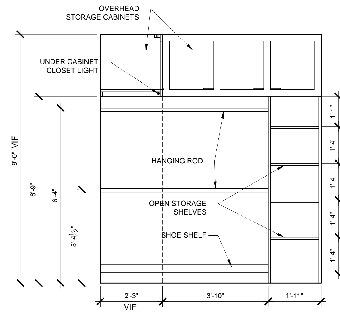
1 CLOSET INTERIOR ELEVATION SCALE: 1/2" = 1'-0"
