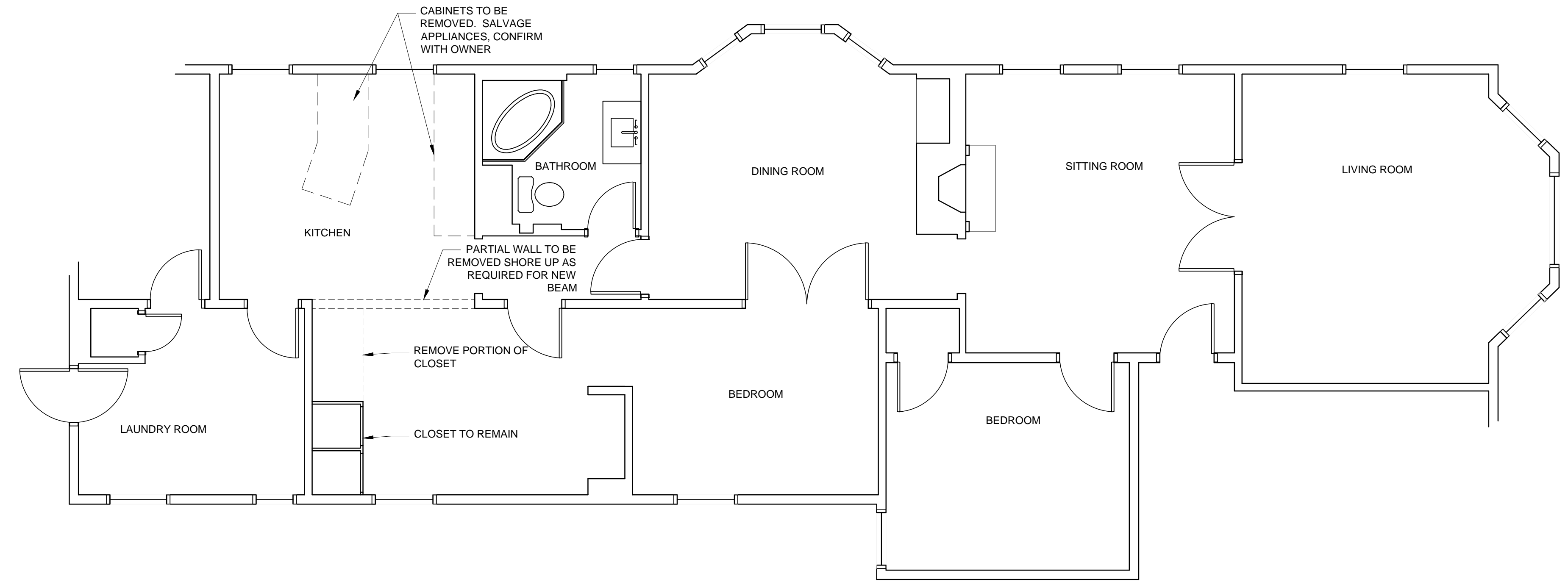
1 EXISTING/DEMO FLOOR PLAN SCALE: 1/4" = 1'-0"
