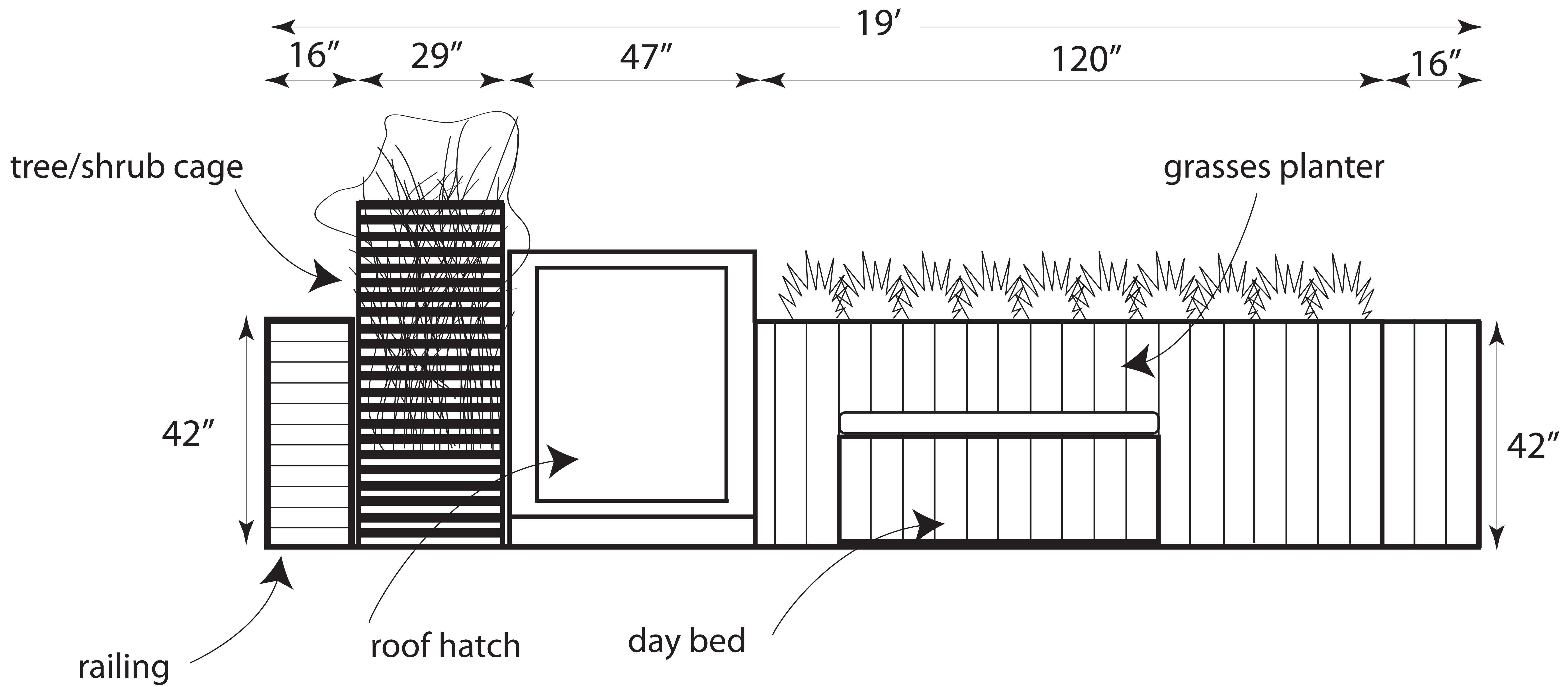
REAR ROOF DECK ELEVATION
