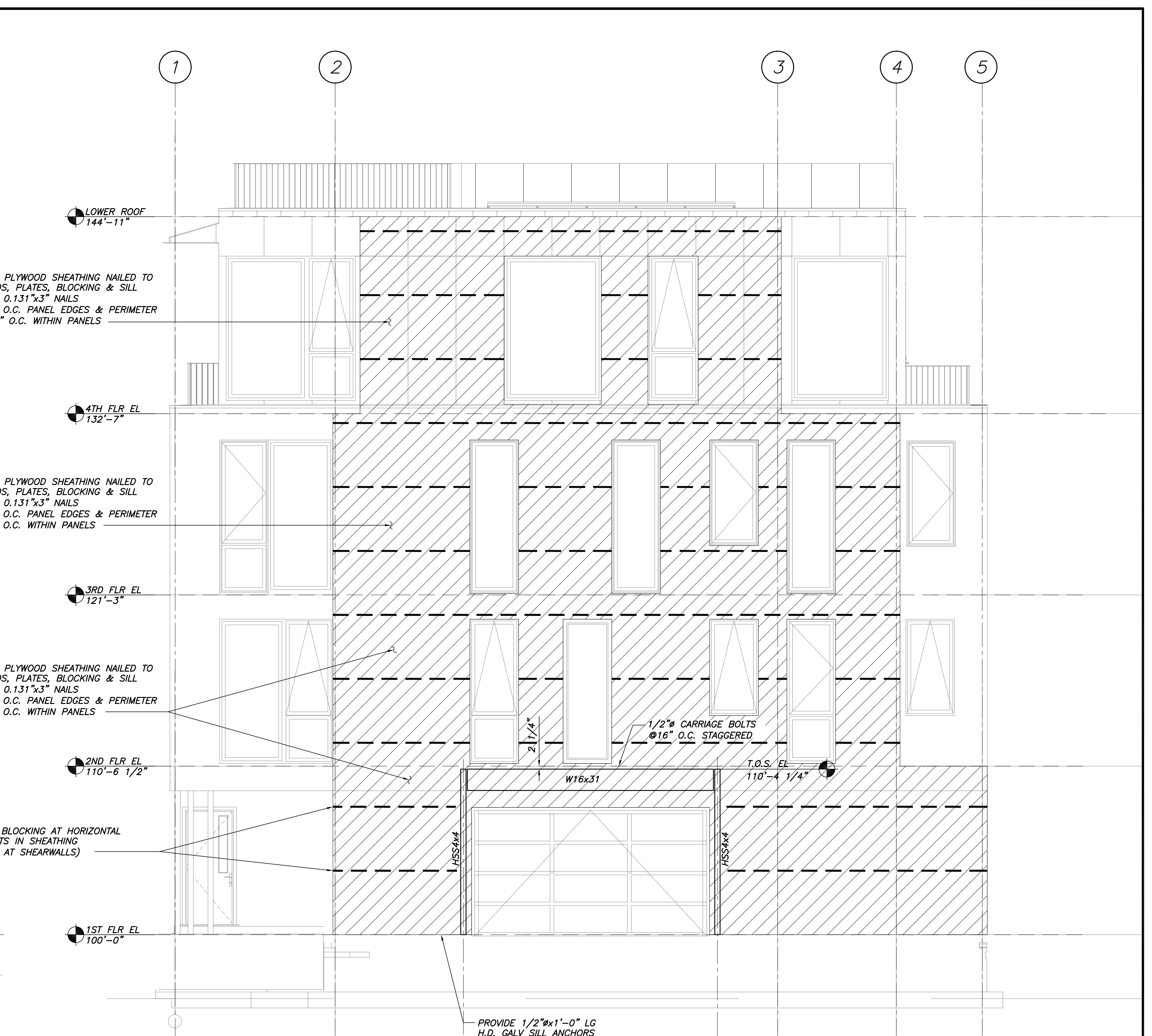
EAST FRAMING ELEVATION 1/4"=1'-0"
