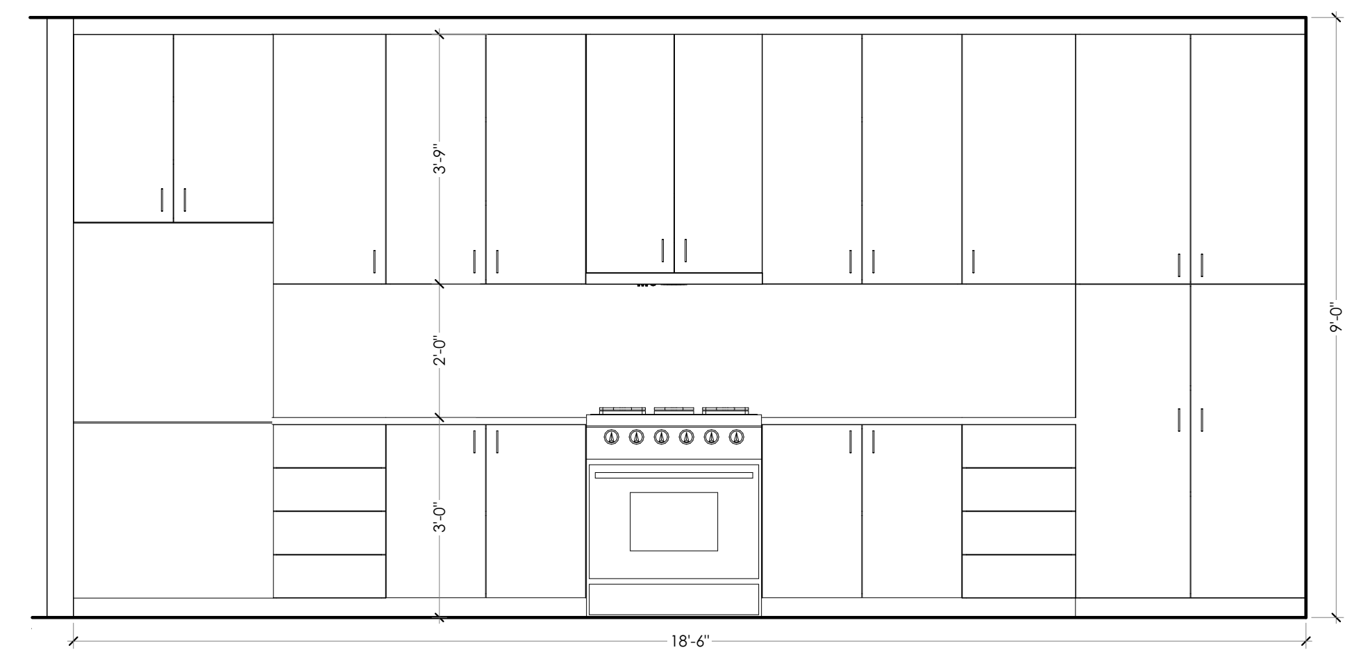
8 TENANT KITCHEN SCALE: 1/2" = 1'-0"
