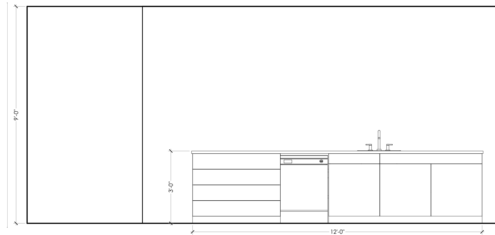
7 ISLAND - RANGE FACING SCALE: 1/2" = 1'-0"
