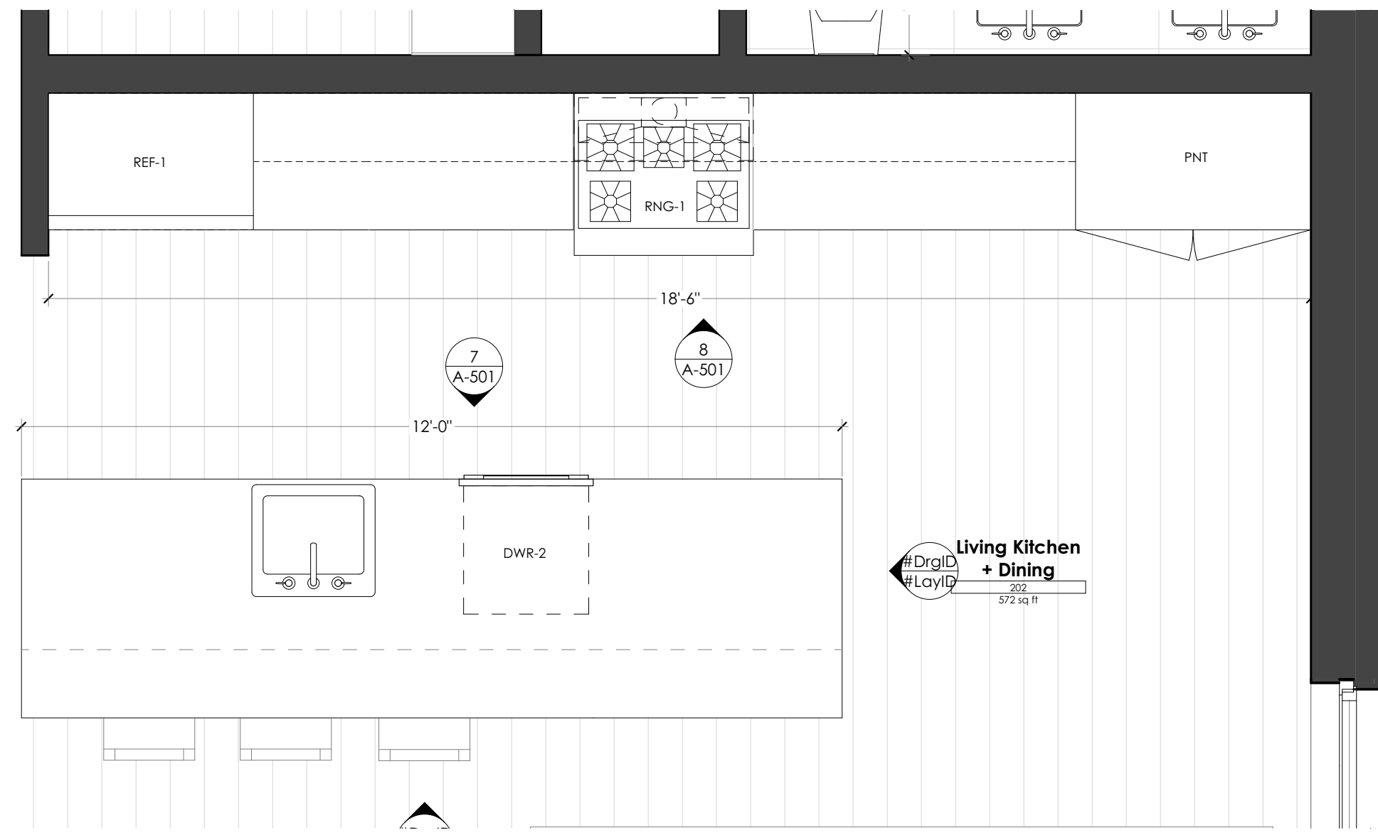
6 2ND FLR ENLARGED PLAN SCALE: 1/2" = 1'-0"
