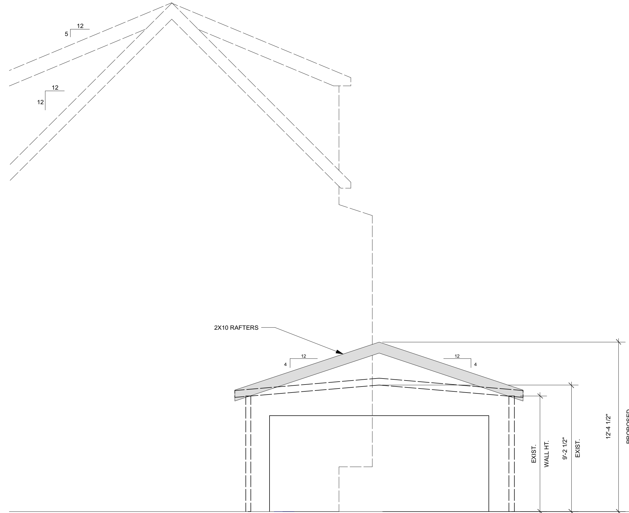
1 PROPOSED GARAGE Scale: 1/4" = 1'-0"
