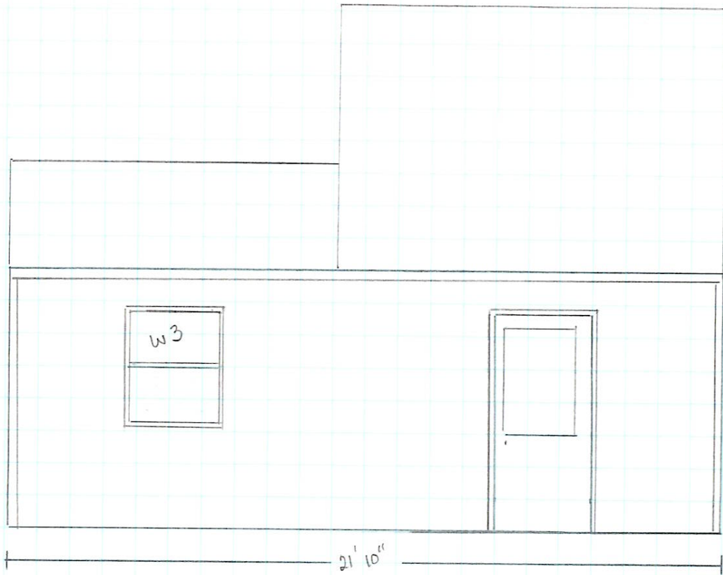
Left Elevation
