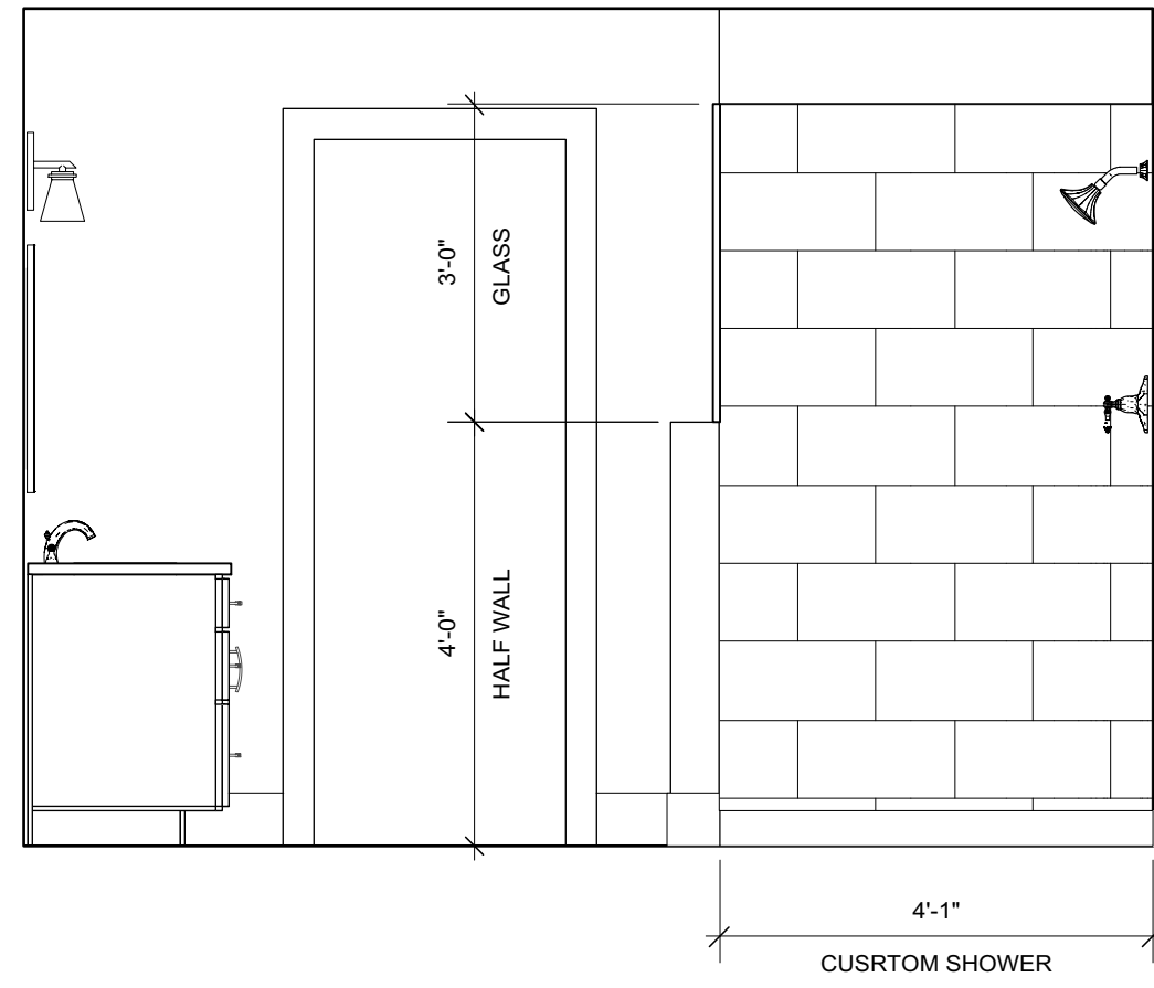
1 MASTER BATH SHOWER Scale: 1/2" = 1'-0"
