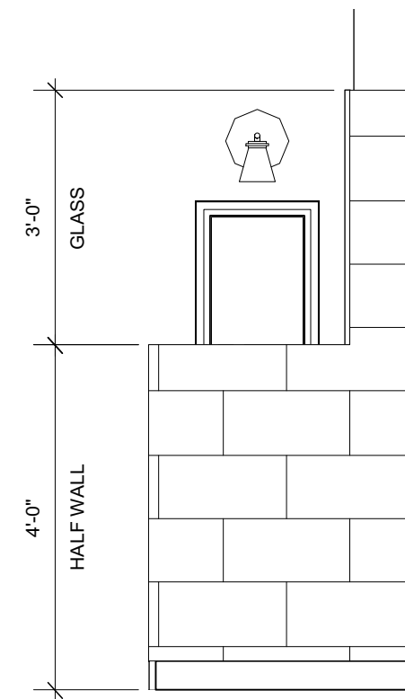
6 MASTER SHOWER: HALF WALL Scale: 1/2" = 1'-0"
