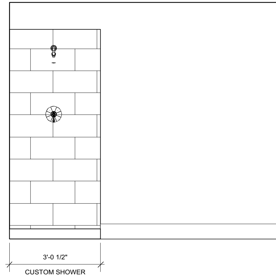
2 MASTER BATH SHOWER Scale: 1/2" = 1'-0"
