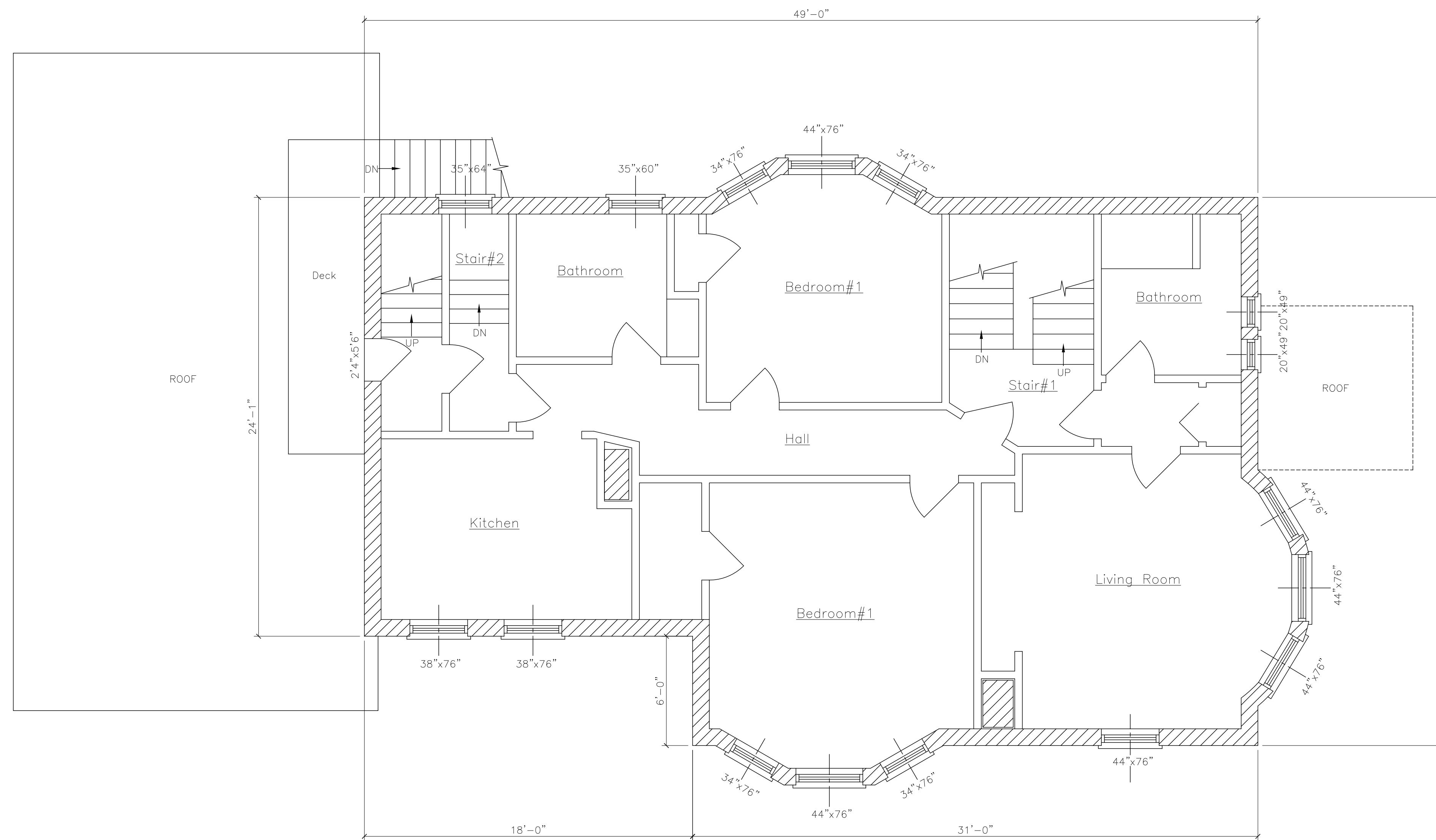
EXISTING FLOOR PLAN—SECOND FLOOR SECOND FLOOR—1432 SQ. FT.
