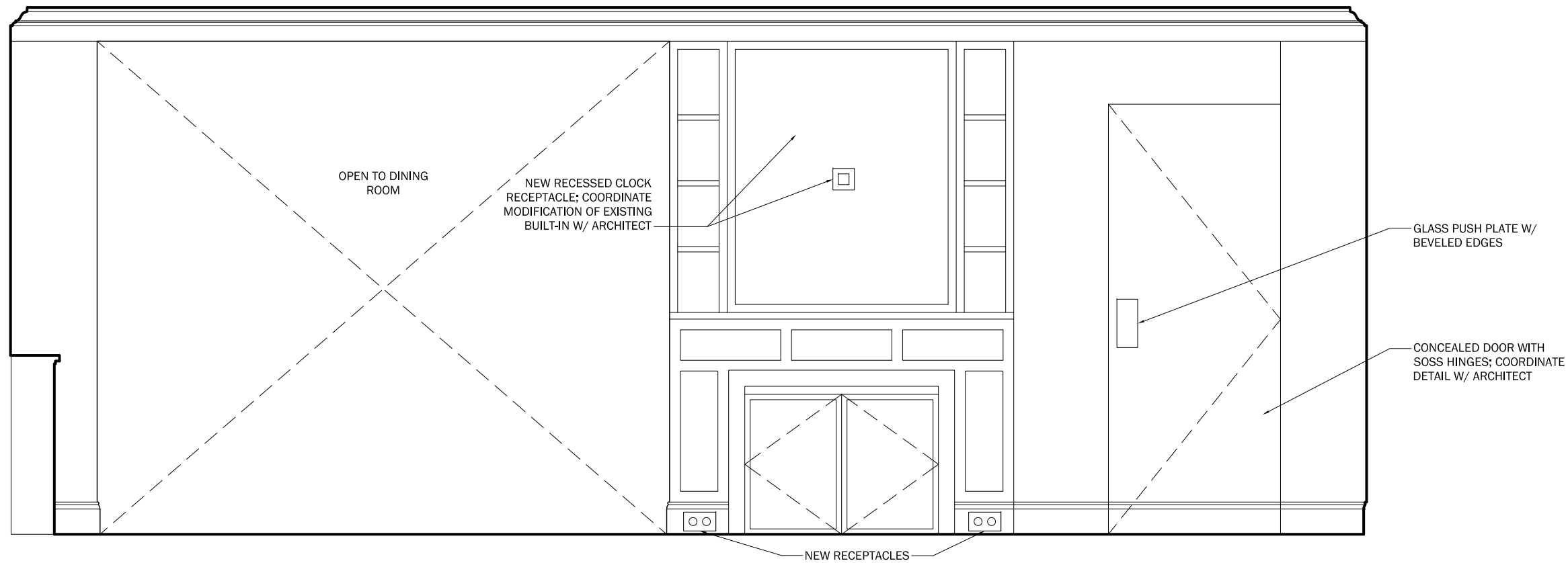
3 LIVING ROOM - WEST \frac{1}{2}'' = 1'-0''
