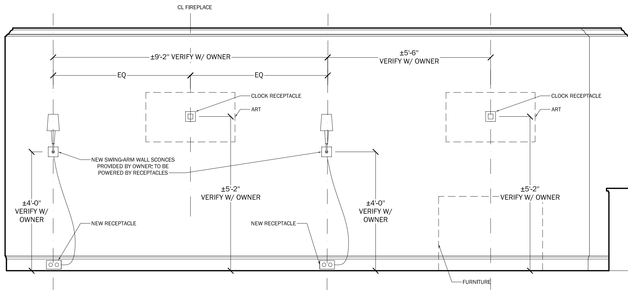
1 LIVING ROOM - EAST \frac{1}{2}'' = 1'-0''
