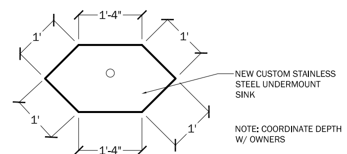
5 KITCHEN SINK DIMENSIONS \frac{1}{2}'' = 1'-0''
