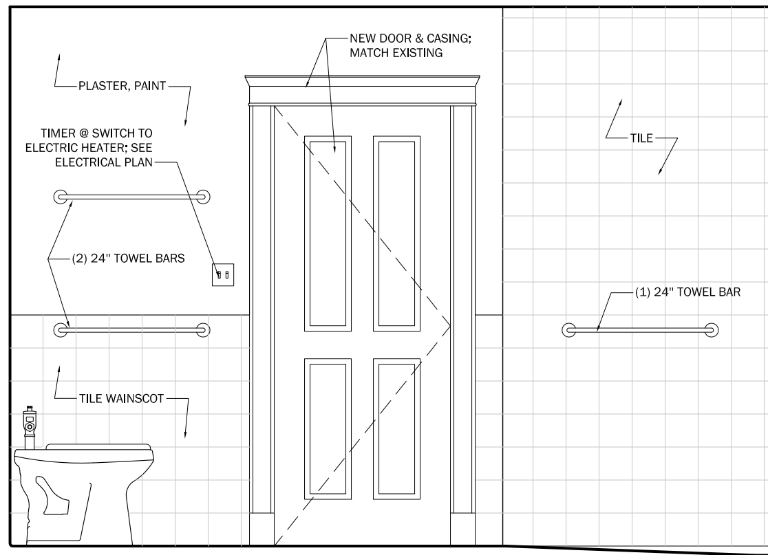
1 JEAN'S BATH - SOUTH 1/2" = 1'-0"
