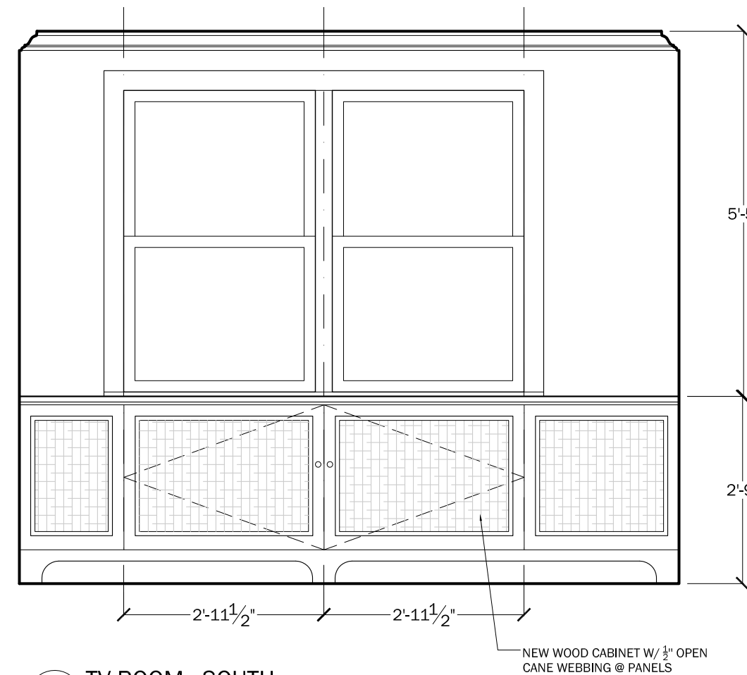
7 TV ROOM - SOUTH 1/2" = 1'-0"
