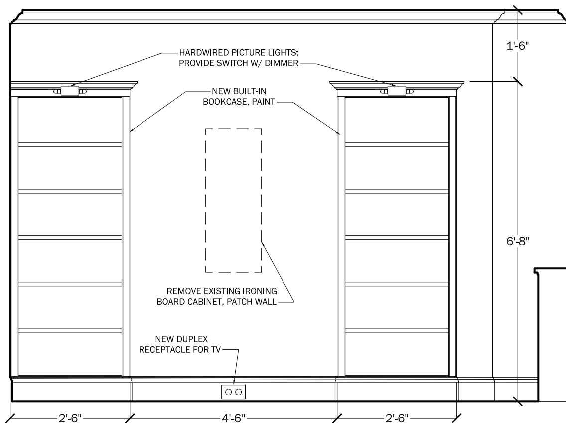
6 TV ROOM - EAST 1/2" = 1'-0"
