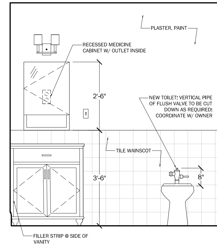
4 JEAN'S BATH - EAST 1/2" = 1'-0"
