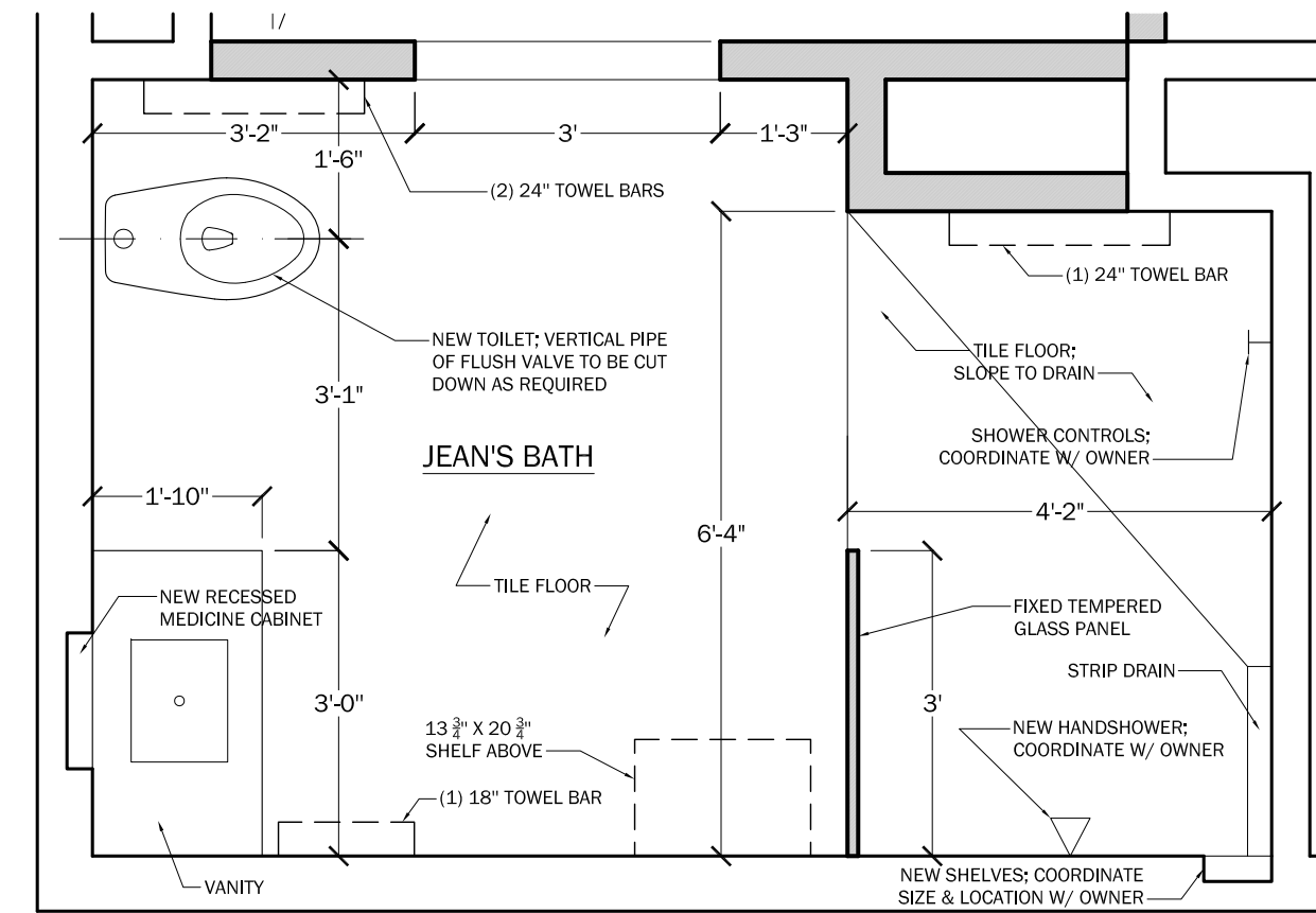
4 JEAN'S BATH - EAST 1/2" = 1'-0"
