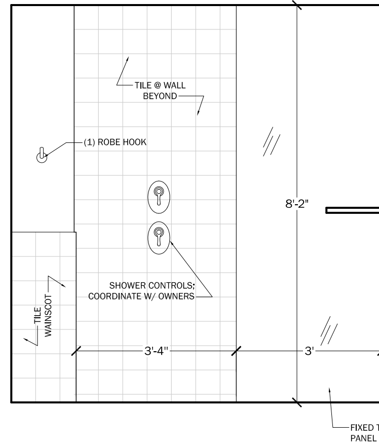
2 JEAN'S BATH - WEST 1/2" = 1'-0"
