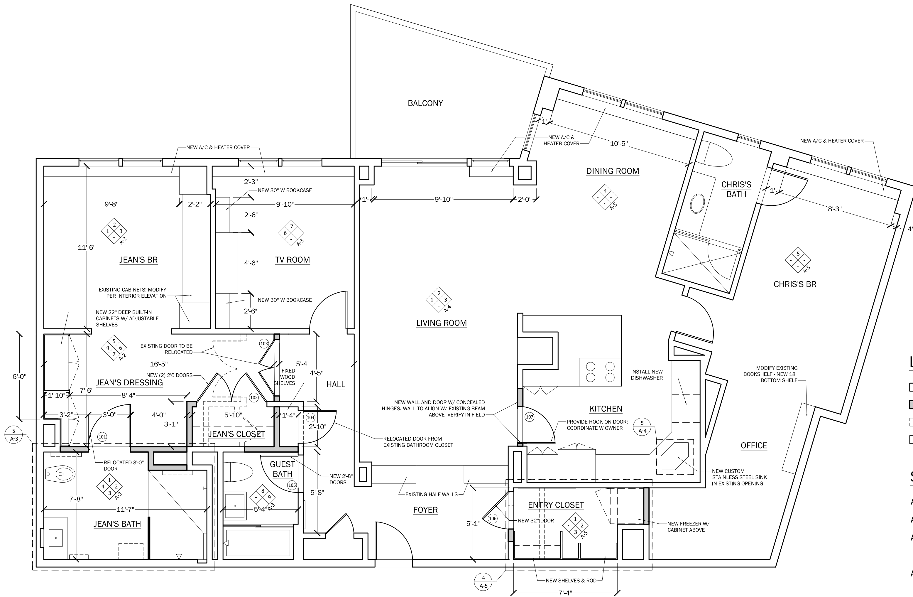
1 FLOOR PLAN \frac{1}{4}'' = 1'-0''
